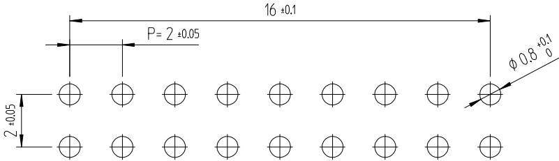
RECOMMENDED LAND PATTERN (FREE) (PCB THICKNESS t=1.6mm)
