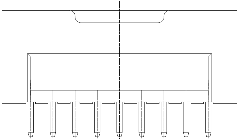
ENGAGEMENT FIGURE (2:1)
