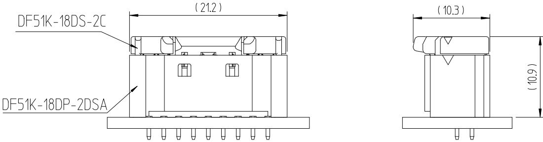
ENGAGEMENT FIGURE (2:1)
