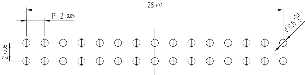
RECOMMENDED LAND PATTERN (FREE) (PCB THICKNESS t=1.6mm)
