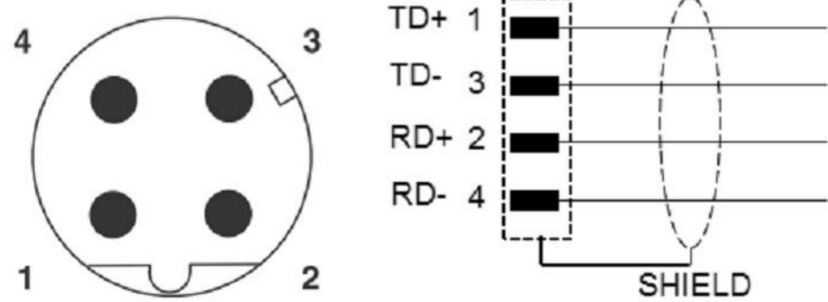
CIRCUIT DIAGRAM MALE
