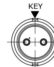
WIRING END ASSY: W6280-2PG-P-3XX SHOWN WITHOUT HARDWARE
