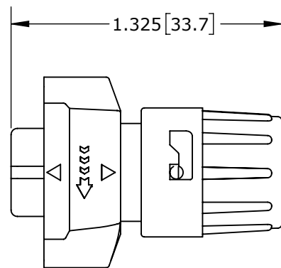
SHOWN ASSEMBLED KIT ASSY: W6280-2PG-P-3XX SHOWN
