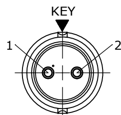
WIRING END W6280-2PG-P-3XX
