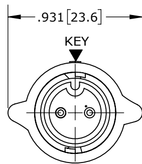
MATING FACE ASSY: W6280-2PG-P-3XX SHOWN
