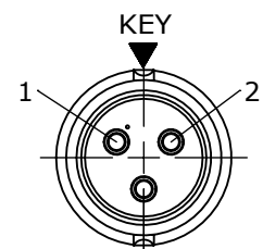
WIRING END W6280-3PG-P-3XX
