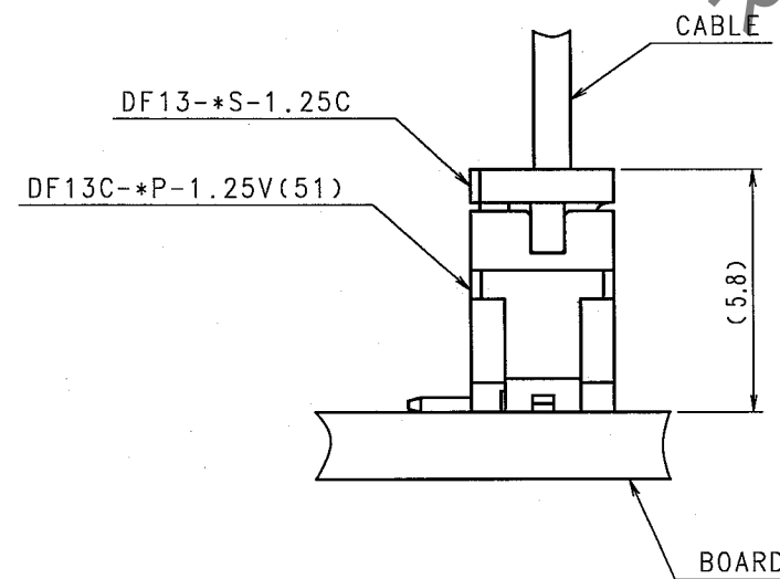
APPLICATION DIAGRAM
