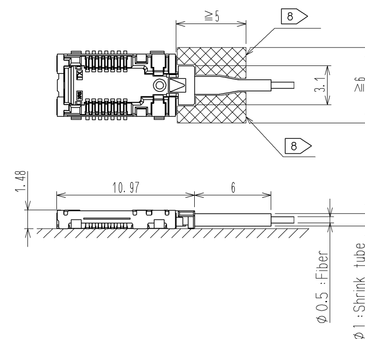
7 Dimensions of engaged connector (Scale : FREE)
