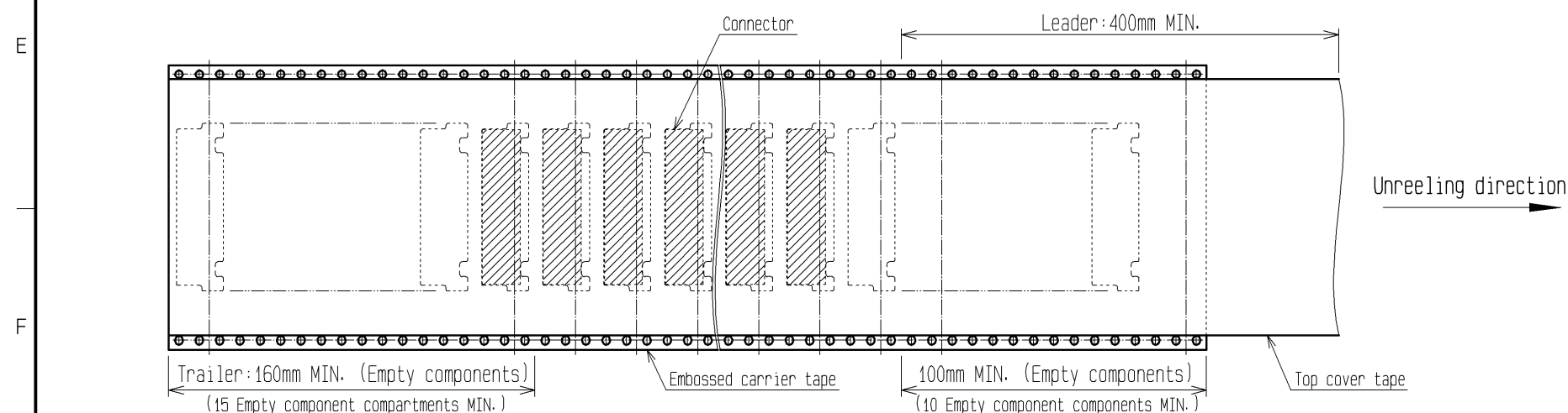
Leader, trailer dimensions (SCALE:FREE)
