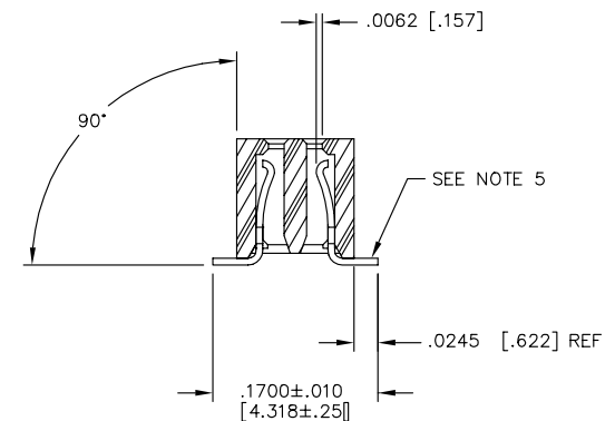
SECT. "B-B"
