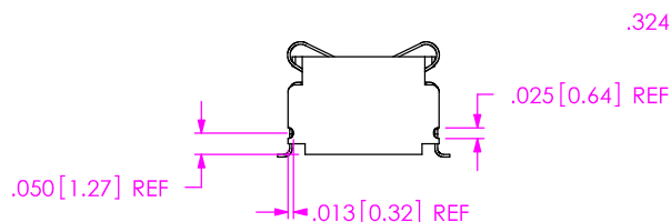
FIG. 1 (FSI-110-06-XXX-D SHOWN)
