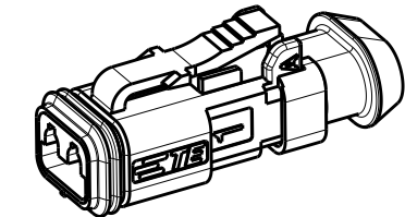
2CCT PLUG CONNECTOR WITH HEATSHRINK HOUSING ULTRASONICALLY WELDED IN PLACE
