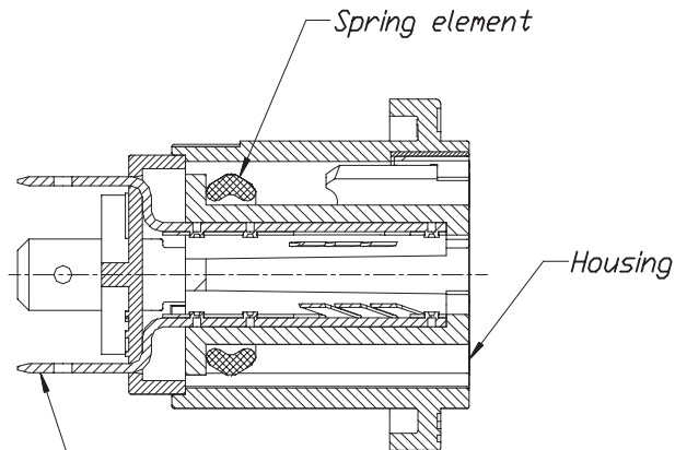
Triple spring loaded contact with Faston termination
