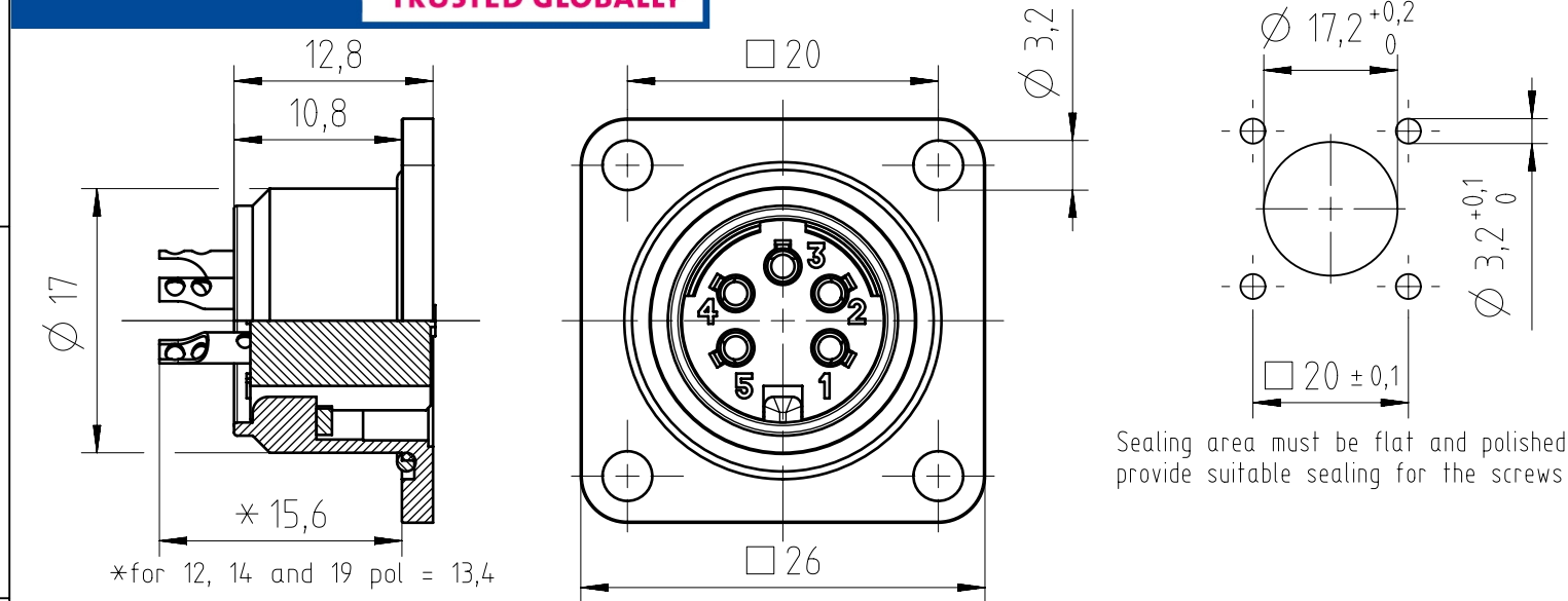
Panel Cutout M1:1
