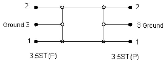
Wiring Diagram
