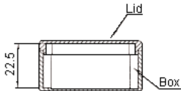
Section on C-C Box and Lid
