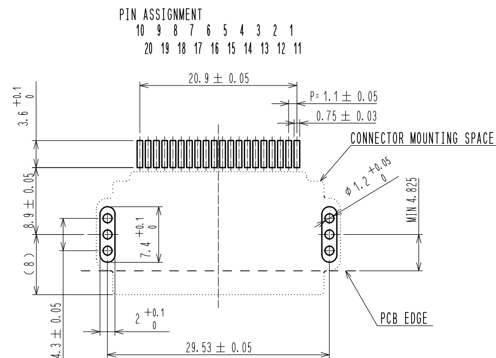
RECOMMENDED PCB PATTERN
