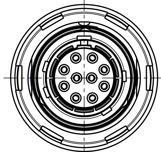
GKT C ATO-E010WN-LS00 Material-ID: 50297054 Mechanical coding: C Color coding: blue
