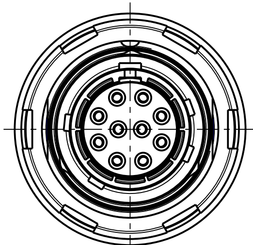
GKT D ATO-E010WN-LS00 Material-ID: 50297055 Mechanical coding: D Color coding: green
