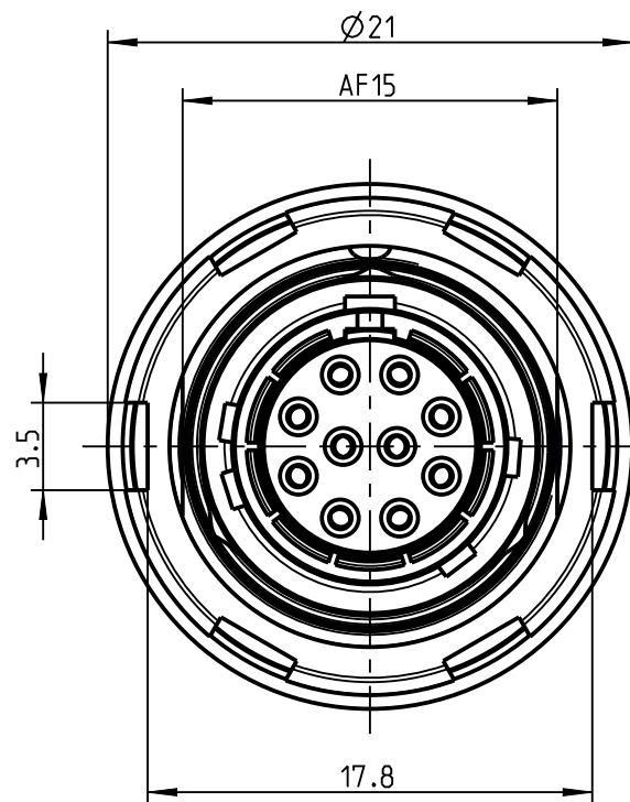
GKT A ATO-E010WN-LS00 Material-ID: 50297050 Mechanical coding: A Color coding: light brown
