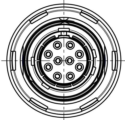
GKT B ATO-E010WN-LS00 Material-ID: 50297051 Mechanical coding: B Color coding: red
