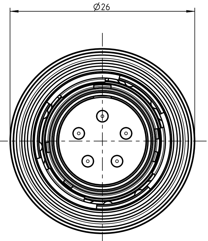
SBTAATO-H005PN-0000 Part-ID: 50298808 Mechanical coding: A Color coding: light brown
