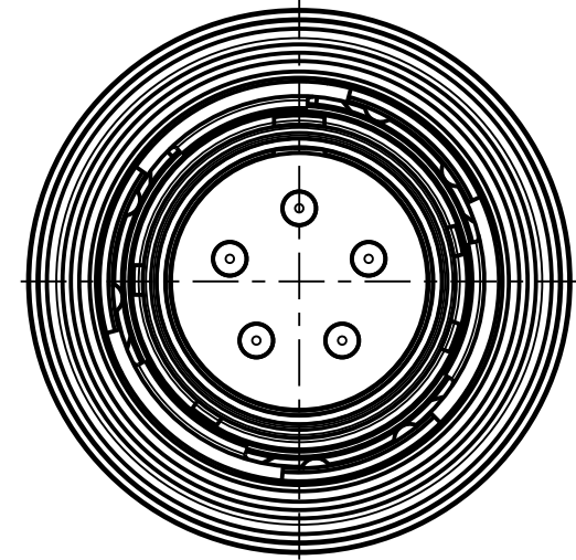
SBTCATO-H005PN-0000 Part-ID: 50298810 Mechanical coding: C Color coding: blue
