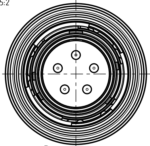
SBTBATO-H005PN-0000 Part-ID: 50298809 Mechanical coding: B Color coding: red
