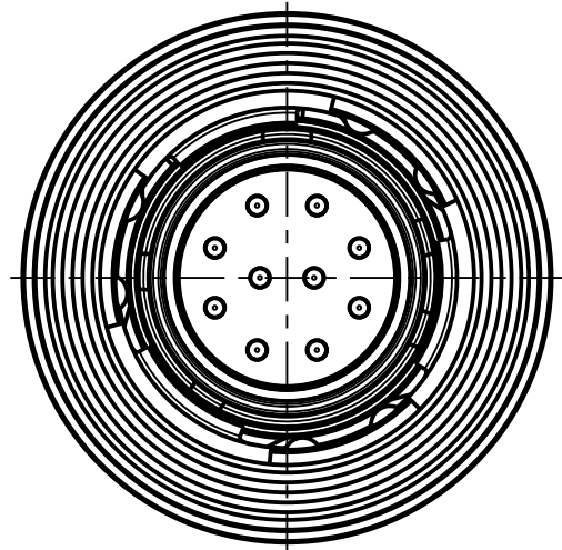
SBTCTATO-E010PN-0000 Material-ID: 50297408 Mechanical coding: C Color coding: blue
