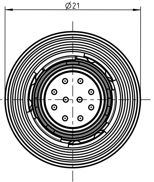
SBTAATO-E010PN-0000 Material-ID: 50297392 Mechanical coding: A Color coding: light brown
