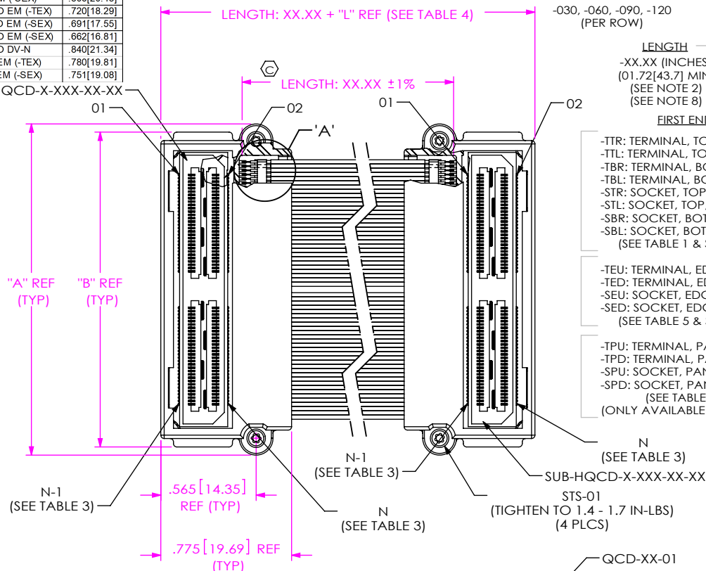
FIG 1 VERTICAL (HQCD-060-XX.XX-STR-STR-1 SHOWN)
