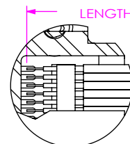
DETAIL 'A' SCALE 2.5 : 1
