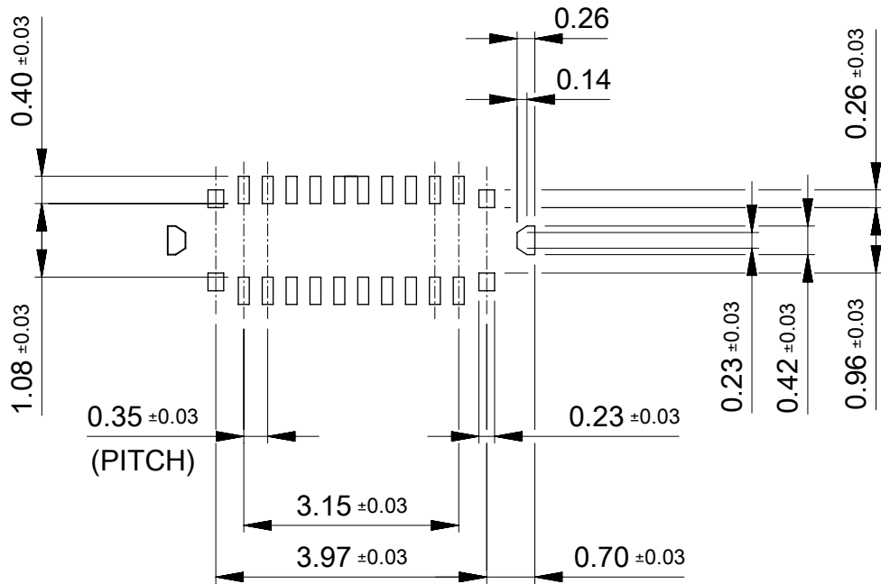
RECOMMENDED METAL MASK LAYOUT (FOR REFERENCE)
