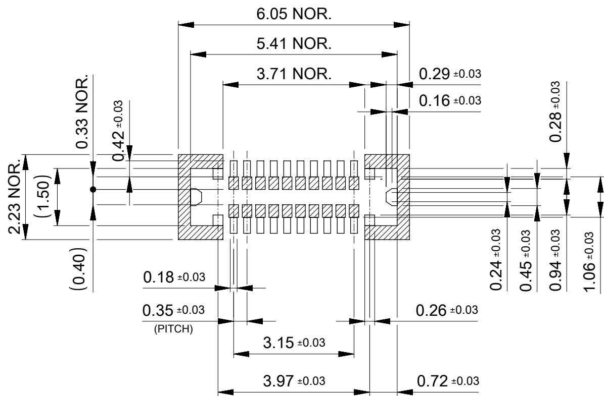
RECOMMENDED P.C.BOARD PATTERN LAYOUT (FOR REFERENCE)
