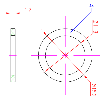
Washer
