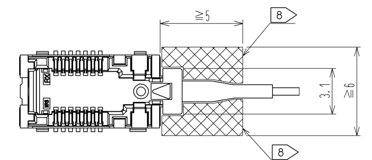
7 Dimensions of engaged connector (Scale:FREE)
