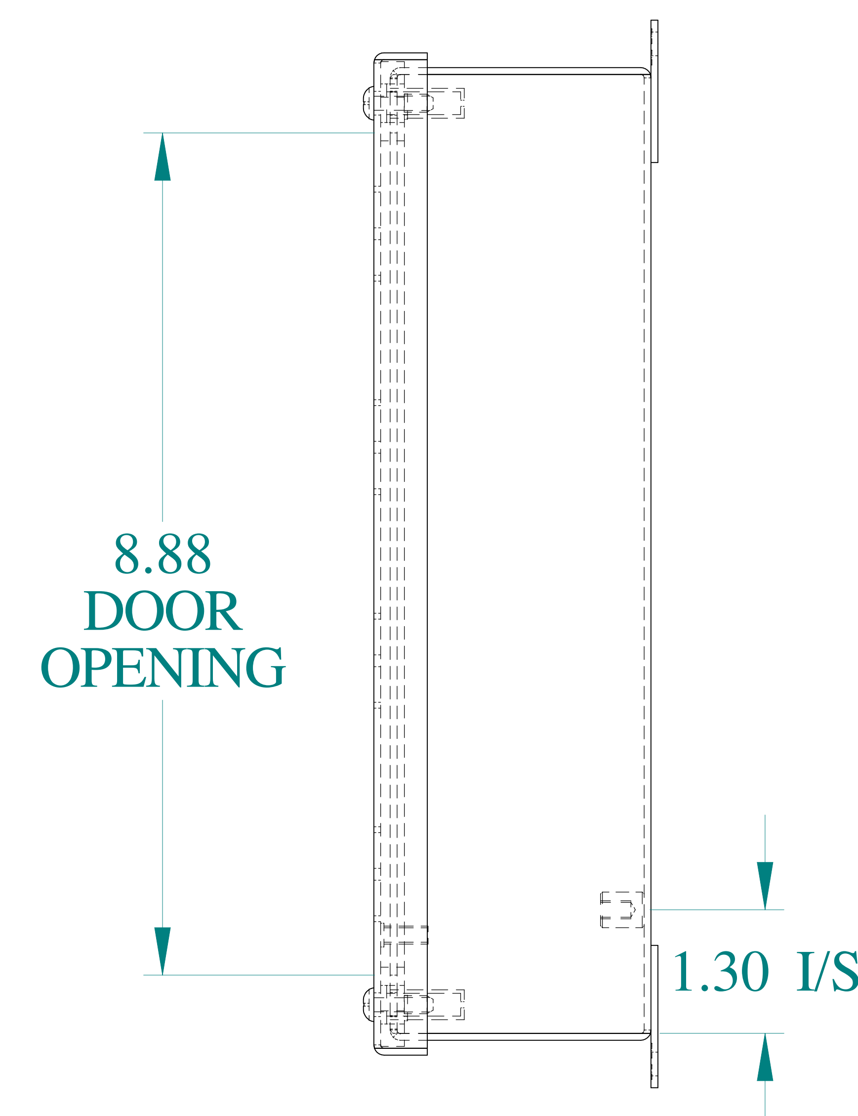
SIDE VIEW
