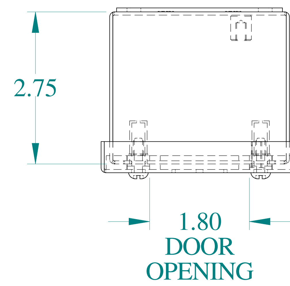
TOP VIEW
