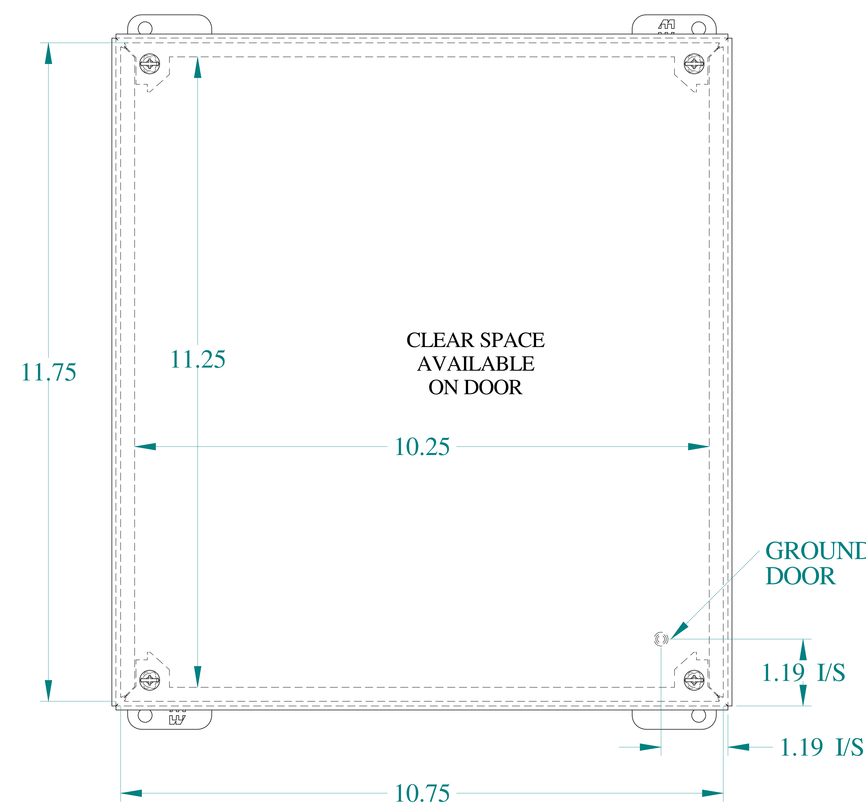
FRONT VIEW
