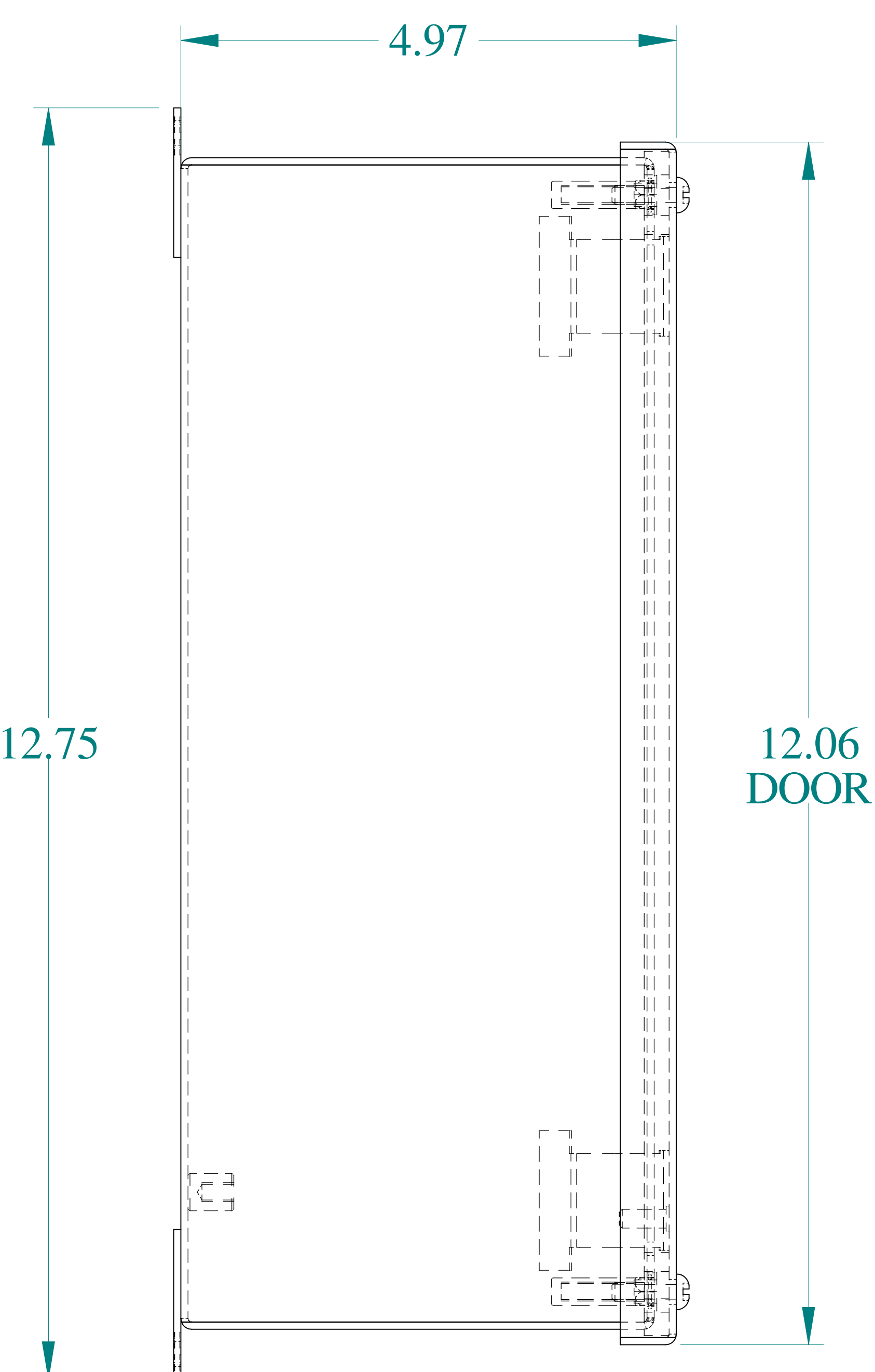
SIDE VIEW
