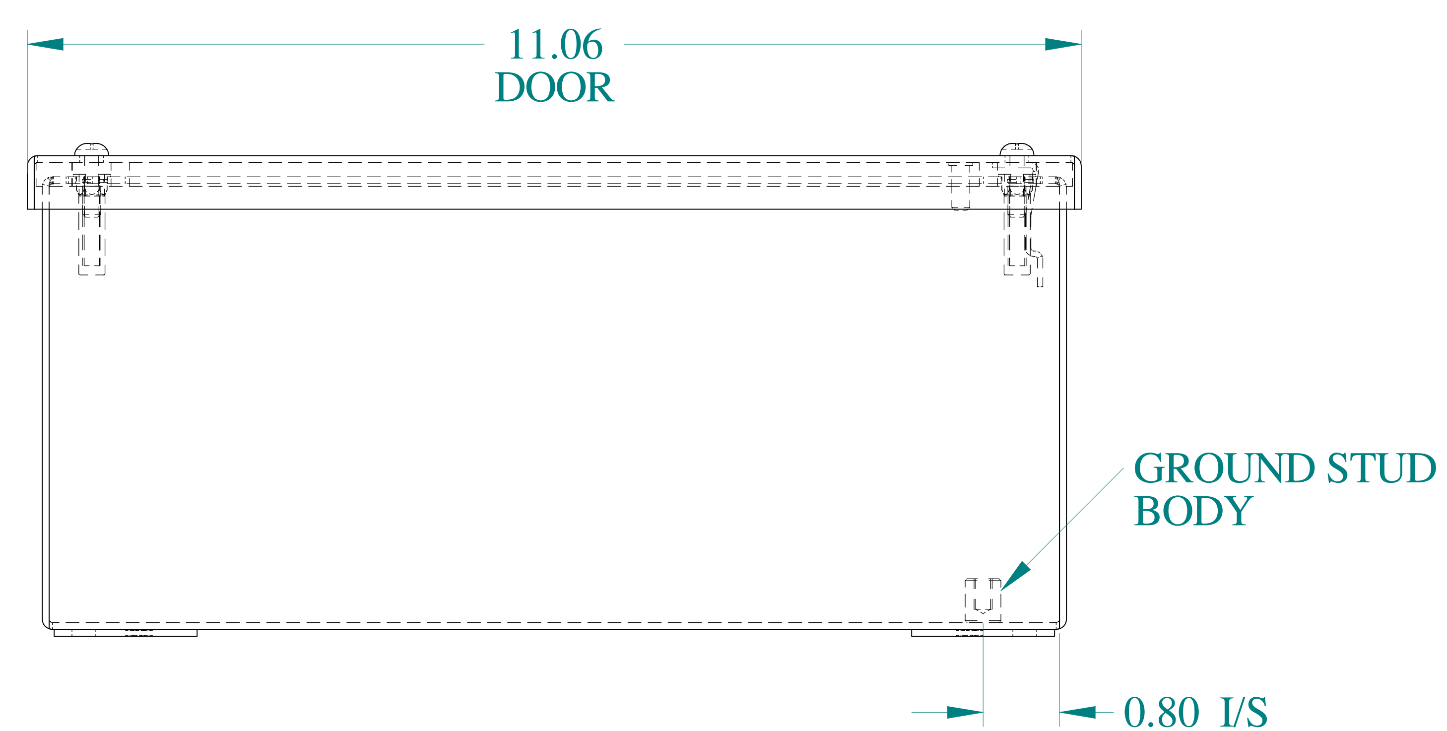
BOTTOM VIEW
