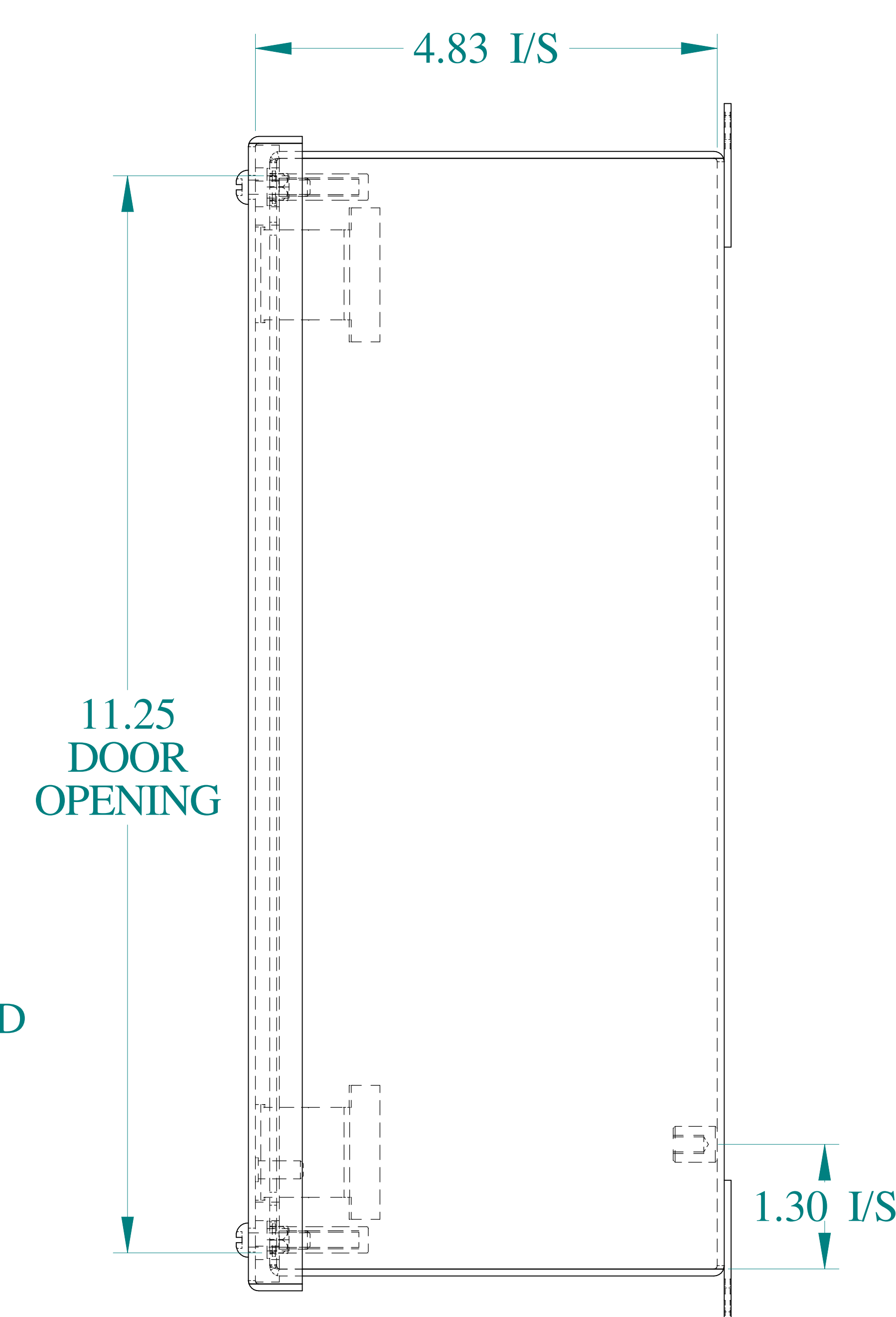
SIDE VIEW
