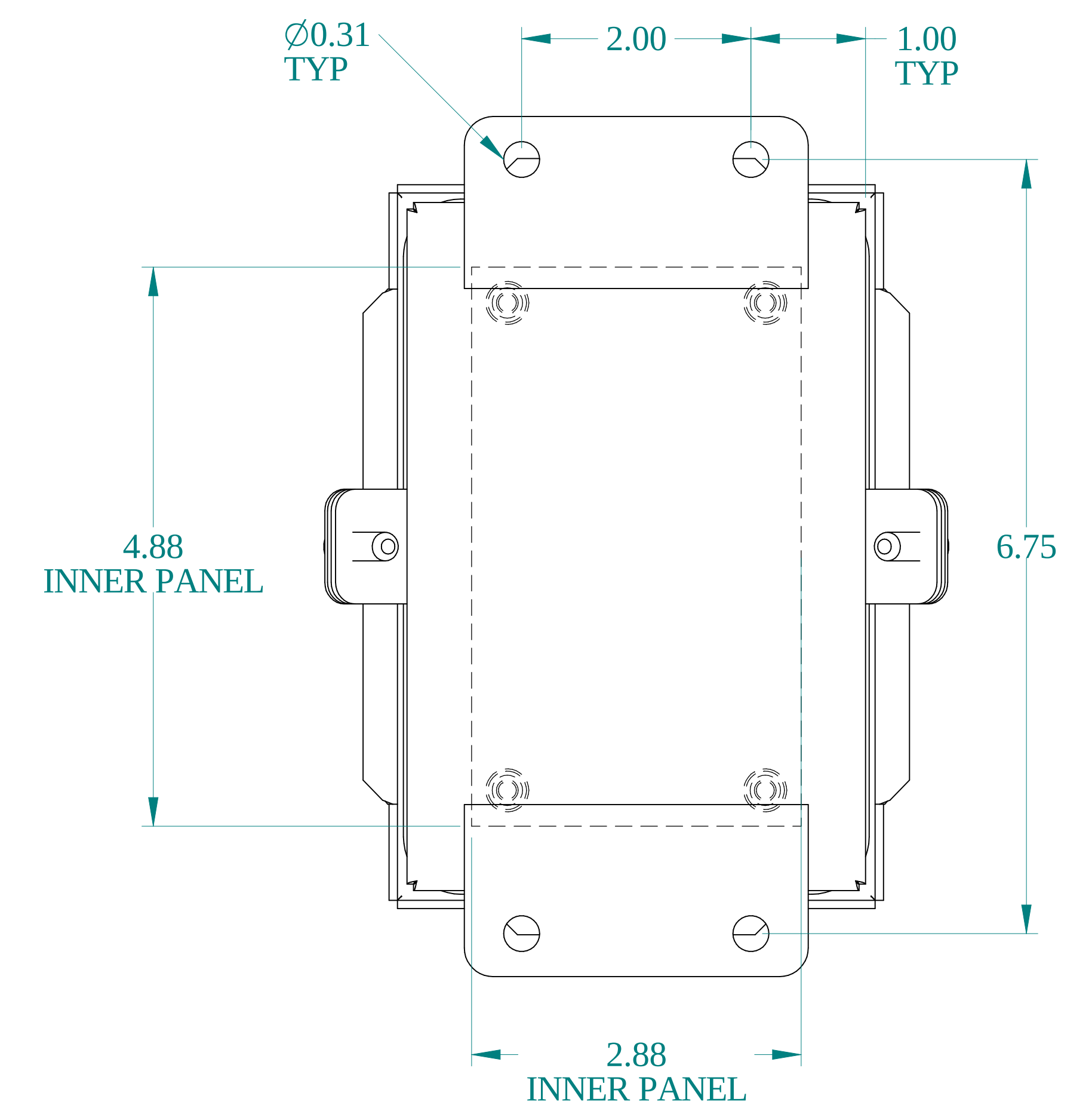
BACK VIEW
