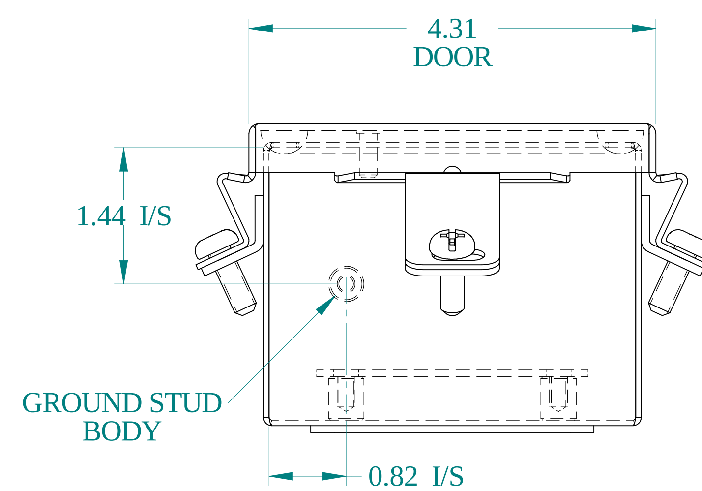
BOTTOM VIEW
