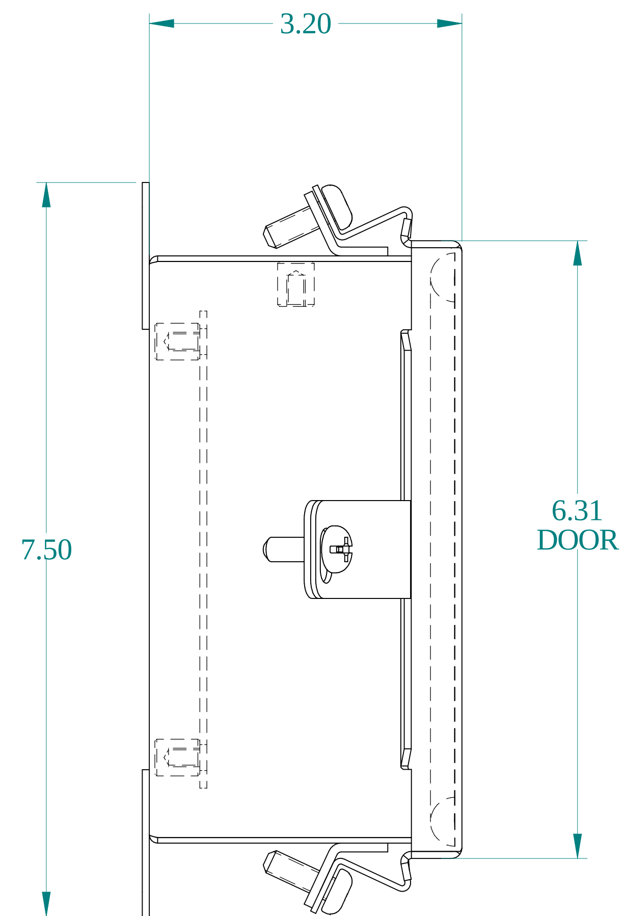
SIDE VIEW
