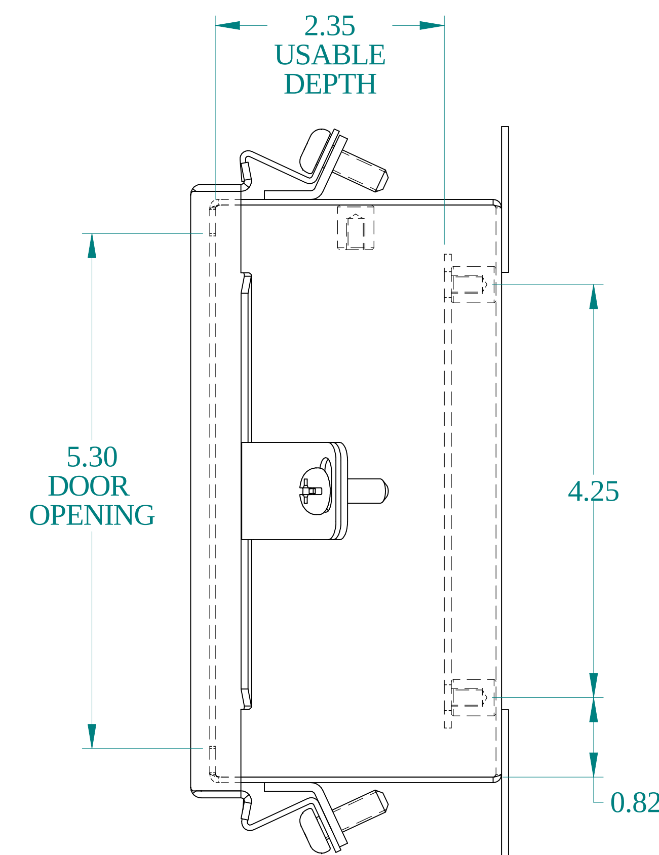
SIDE VIEW
