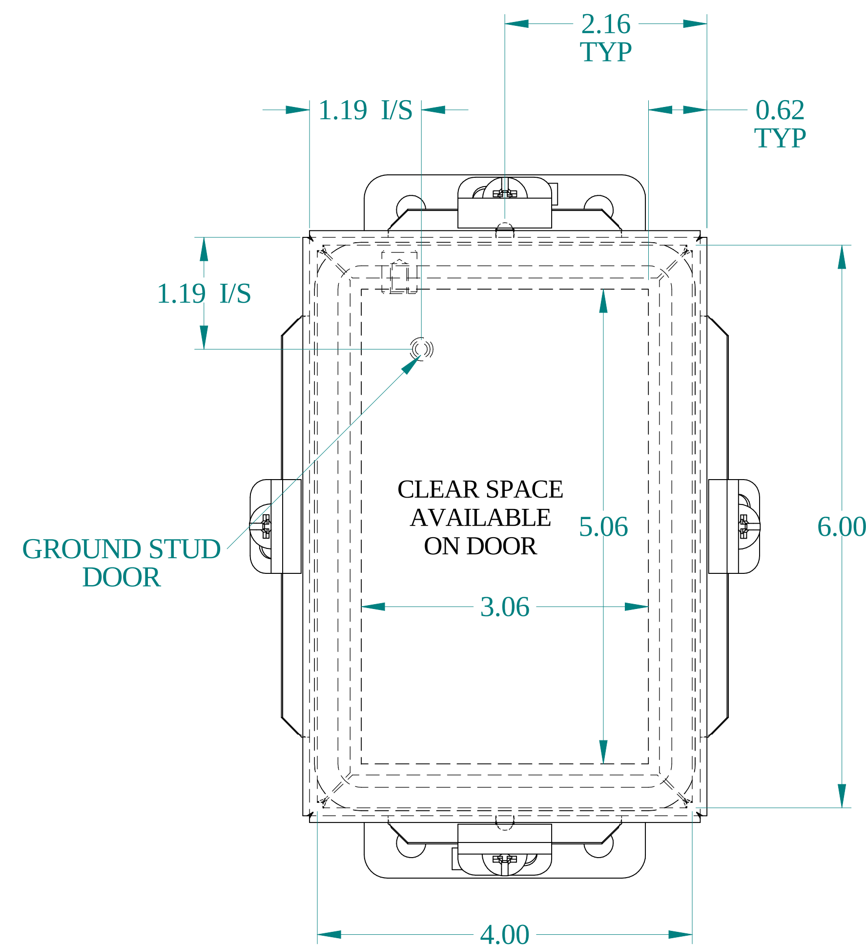
FRONT VIEW
