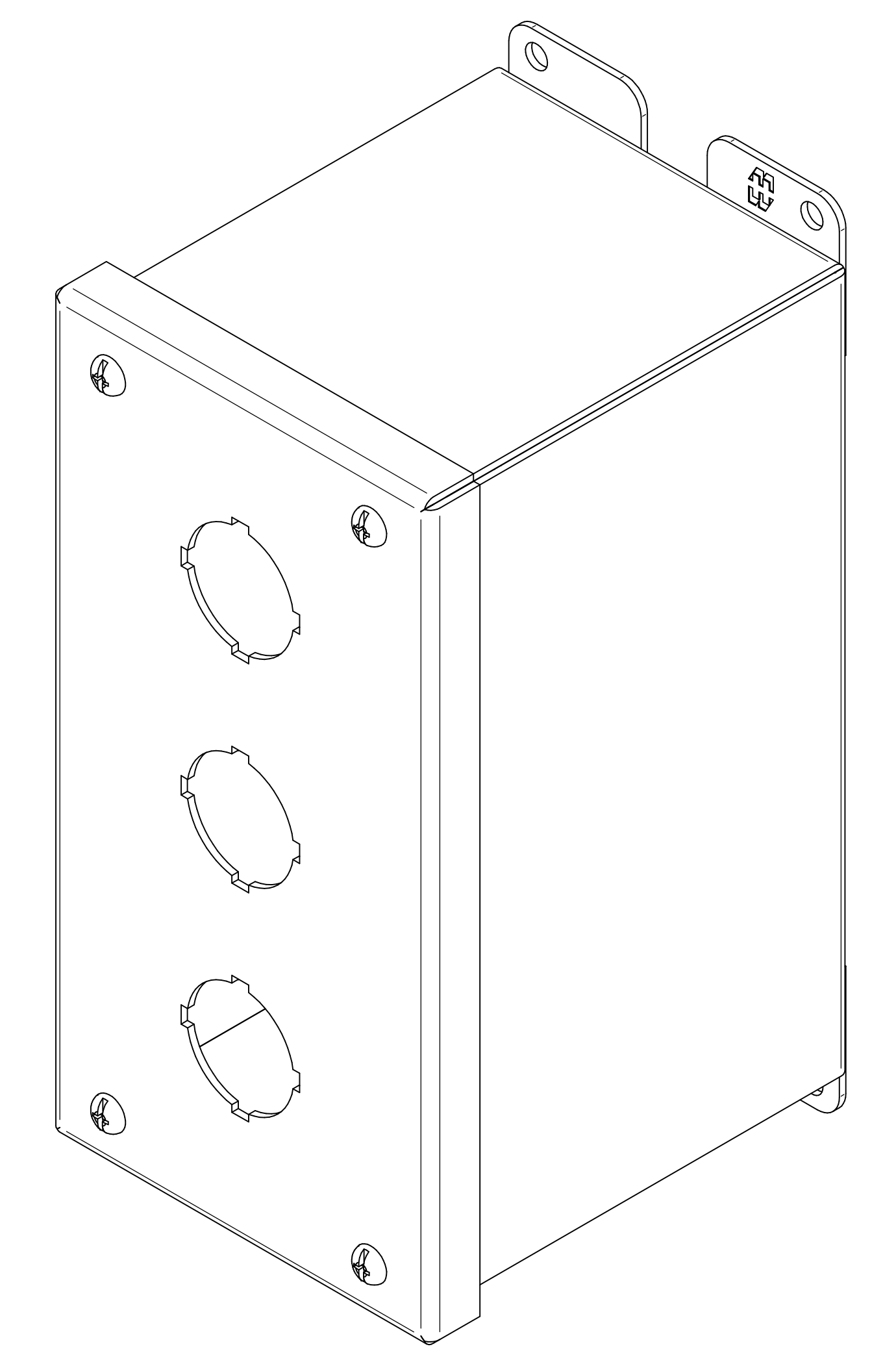
ISOMETRIC VIEWS
