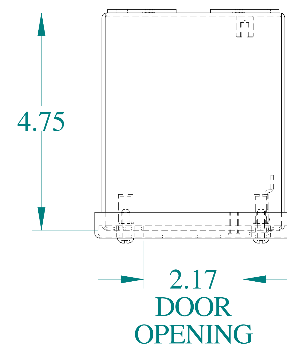
TOP VIEW
