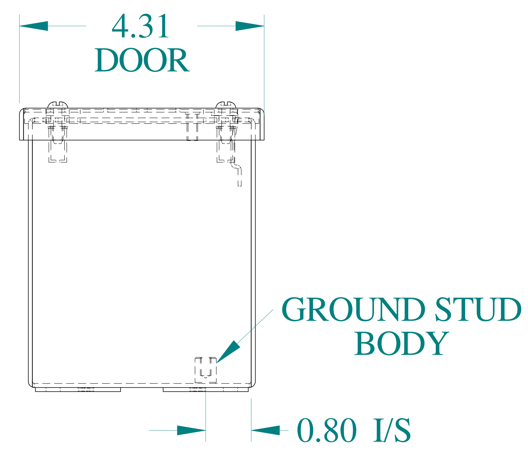
BOTTOM VIEW
