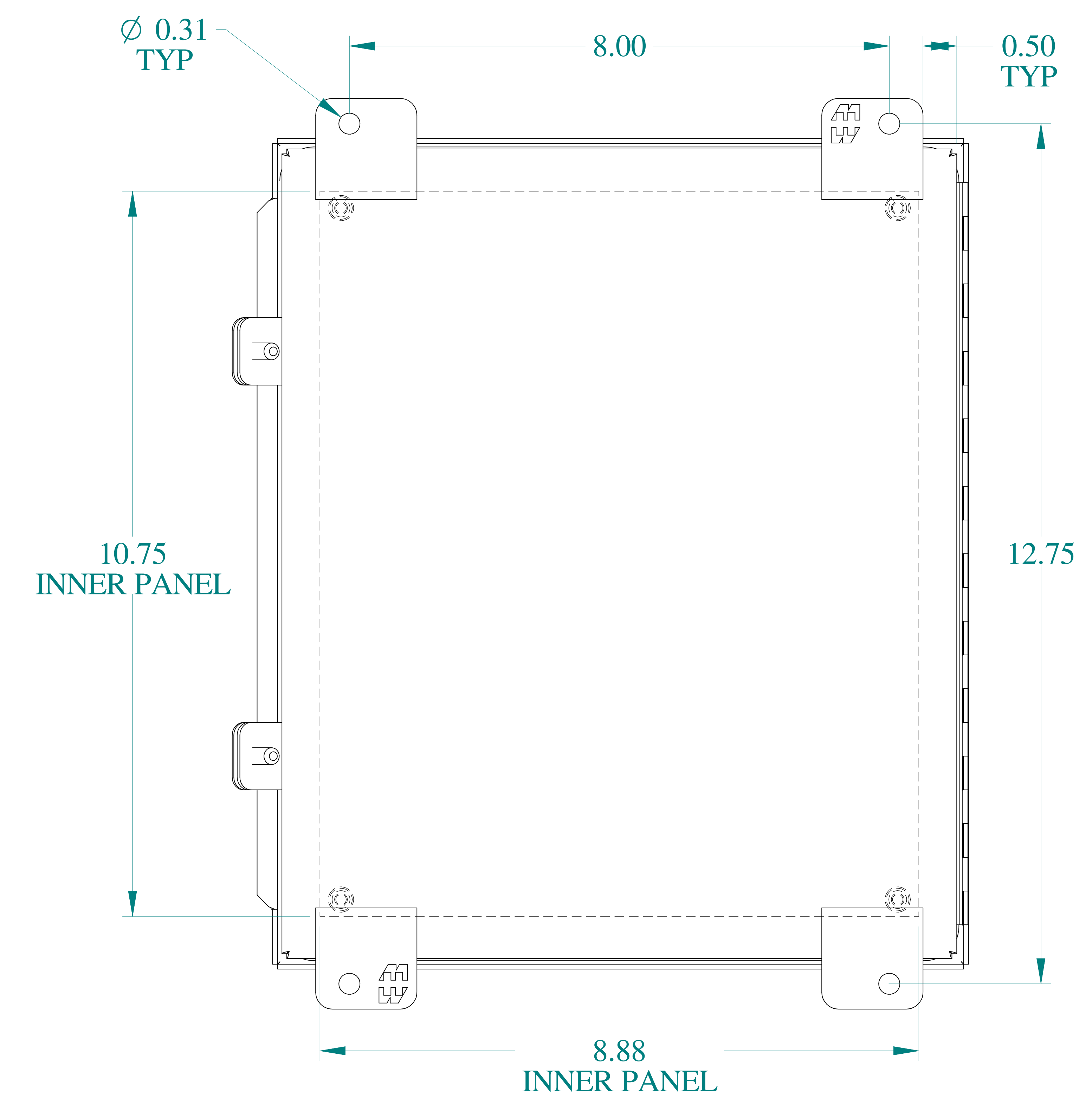
BACK VIEW
