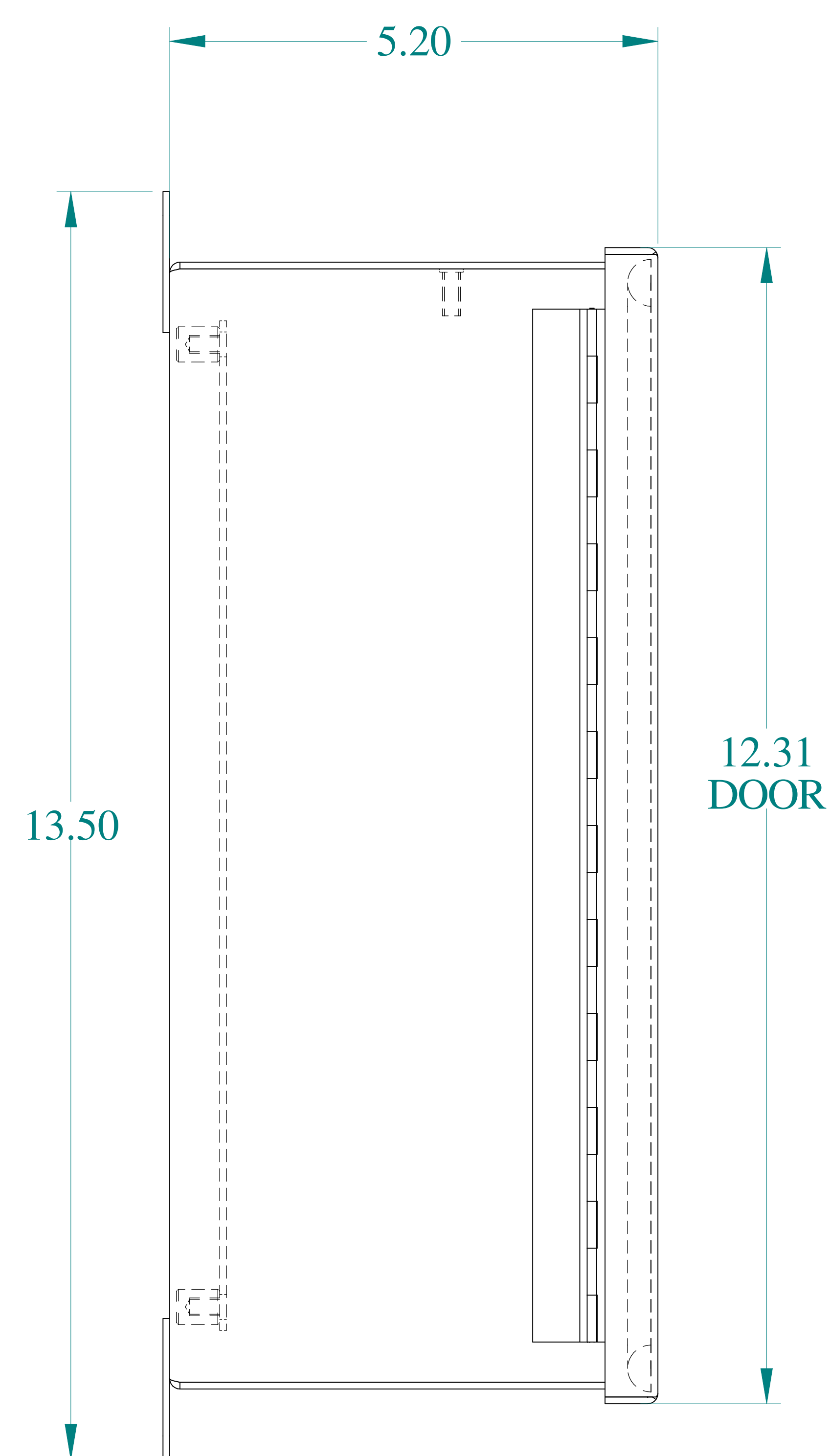
SIDE VIEW
