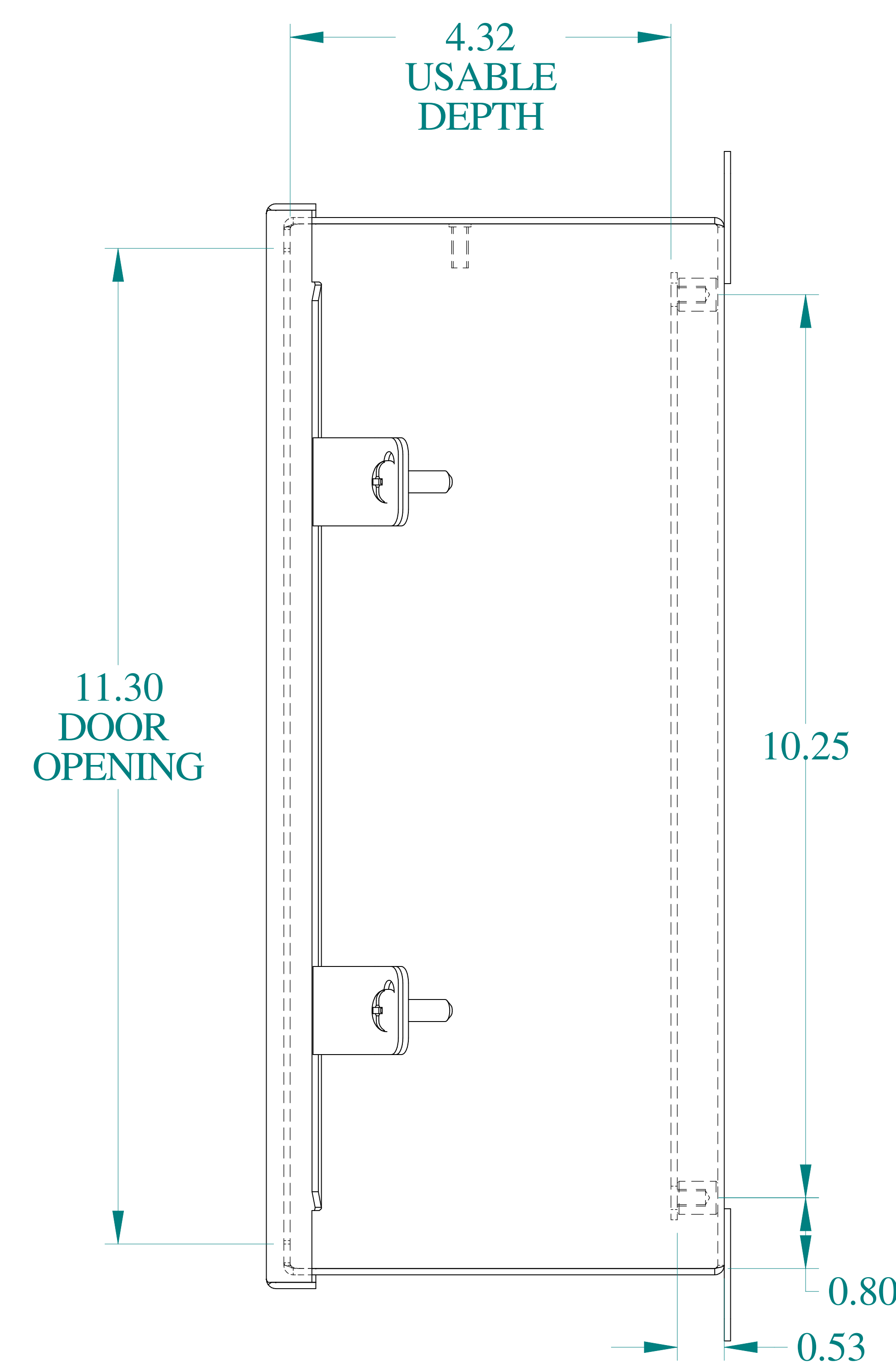
SIDE VIEW
