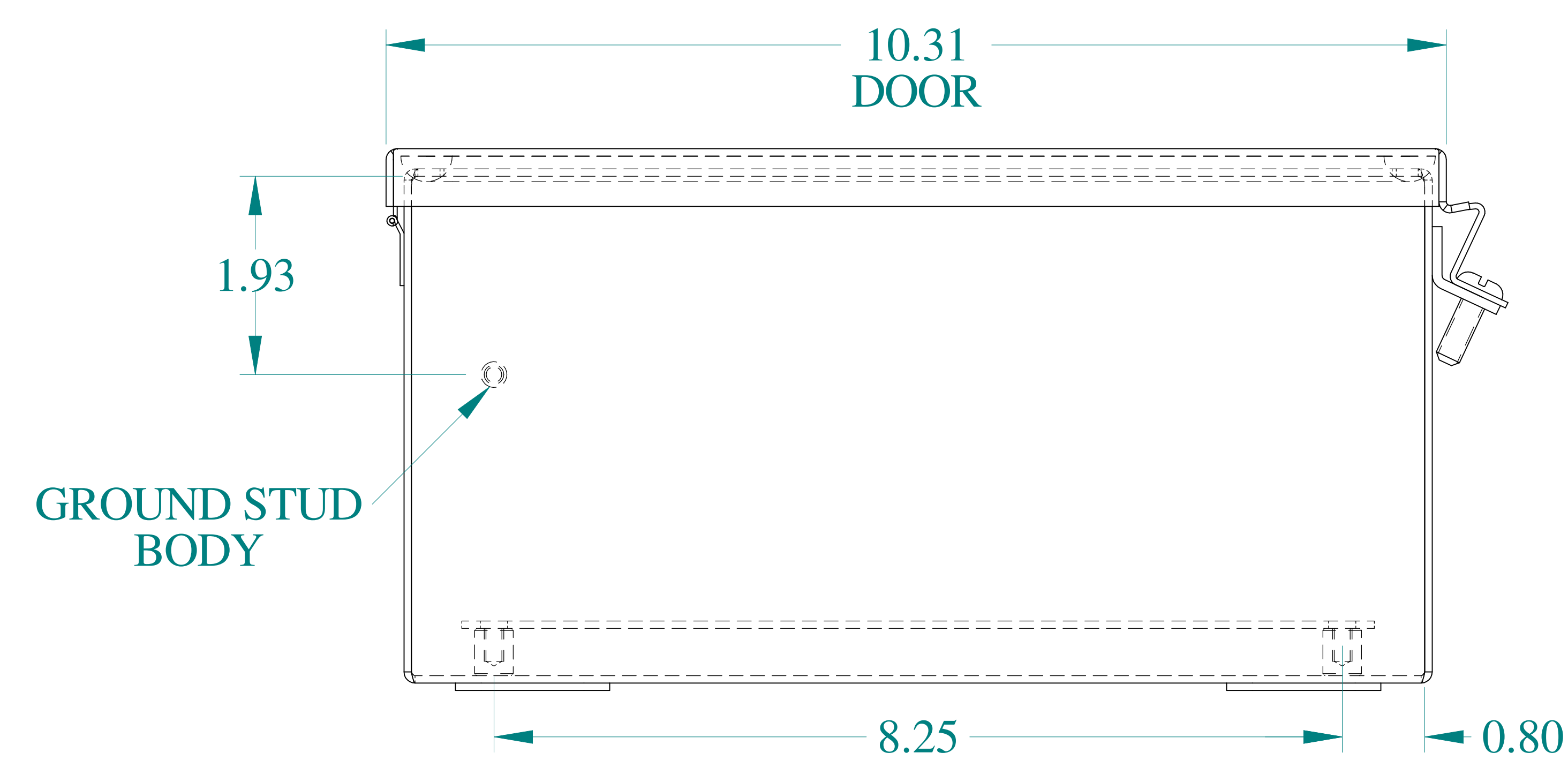
BOTTOM VIEW
