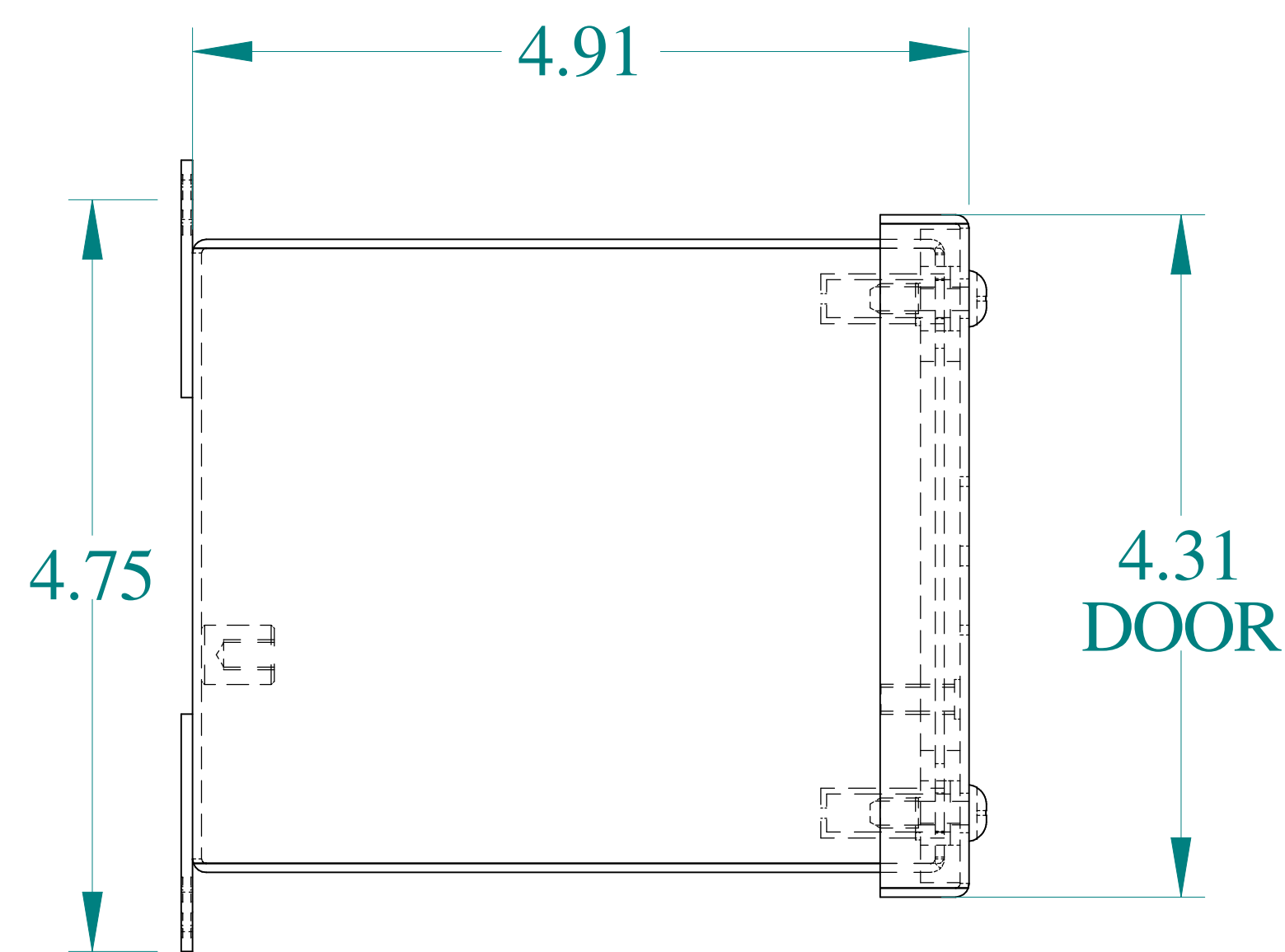
SIDE VIEW
