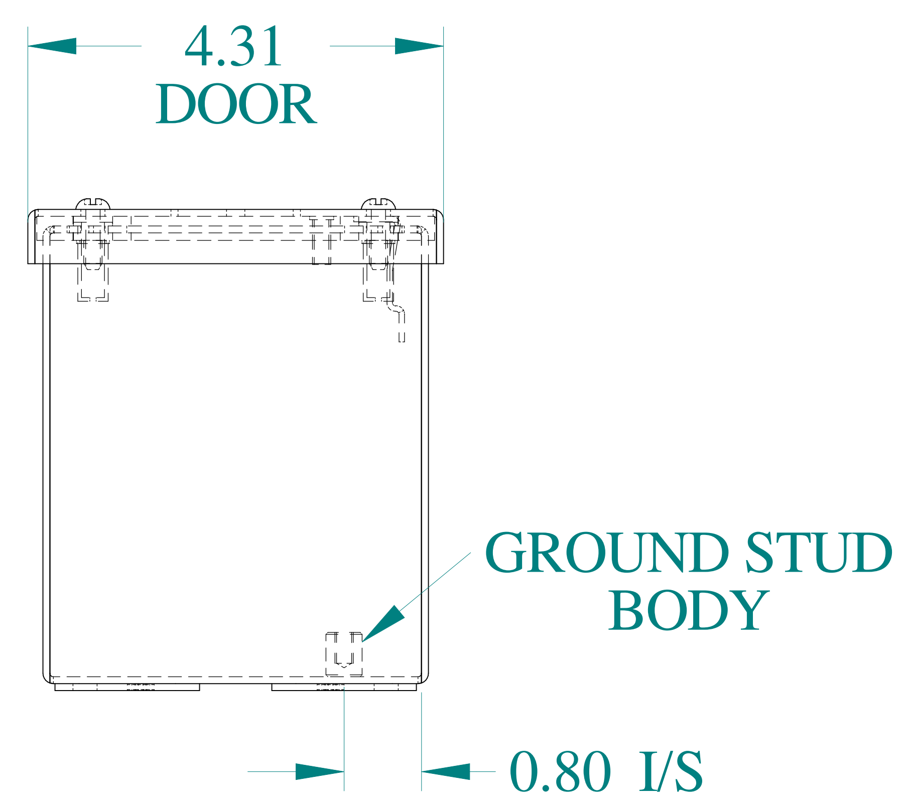
BOTTOM VIEW
