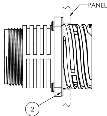
REAR MOUNTING
