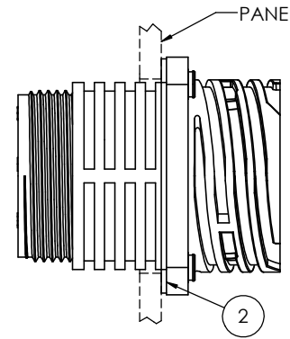
FRONT MOUNTING
