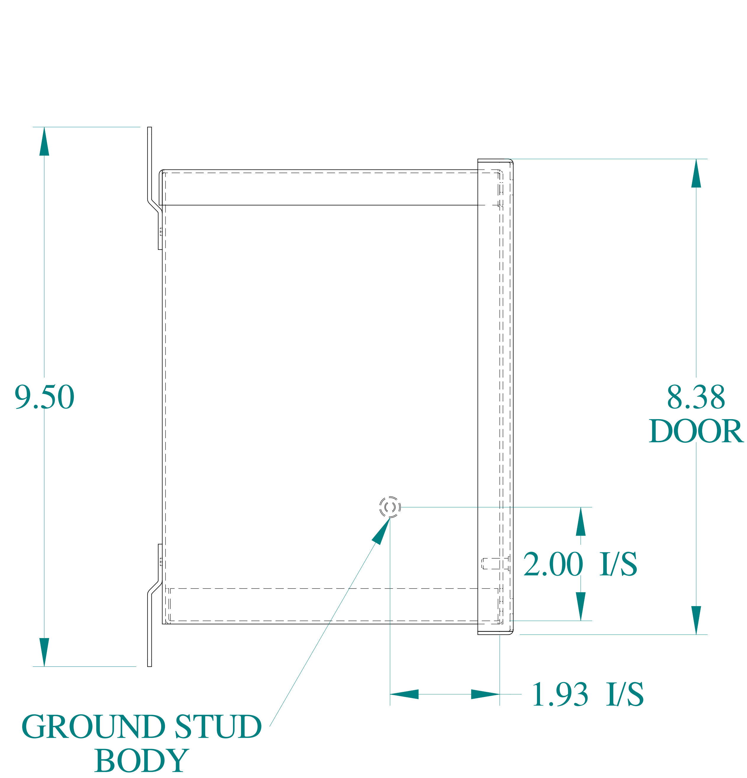
SIDE VIEW
