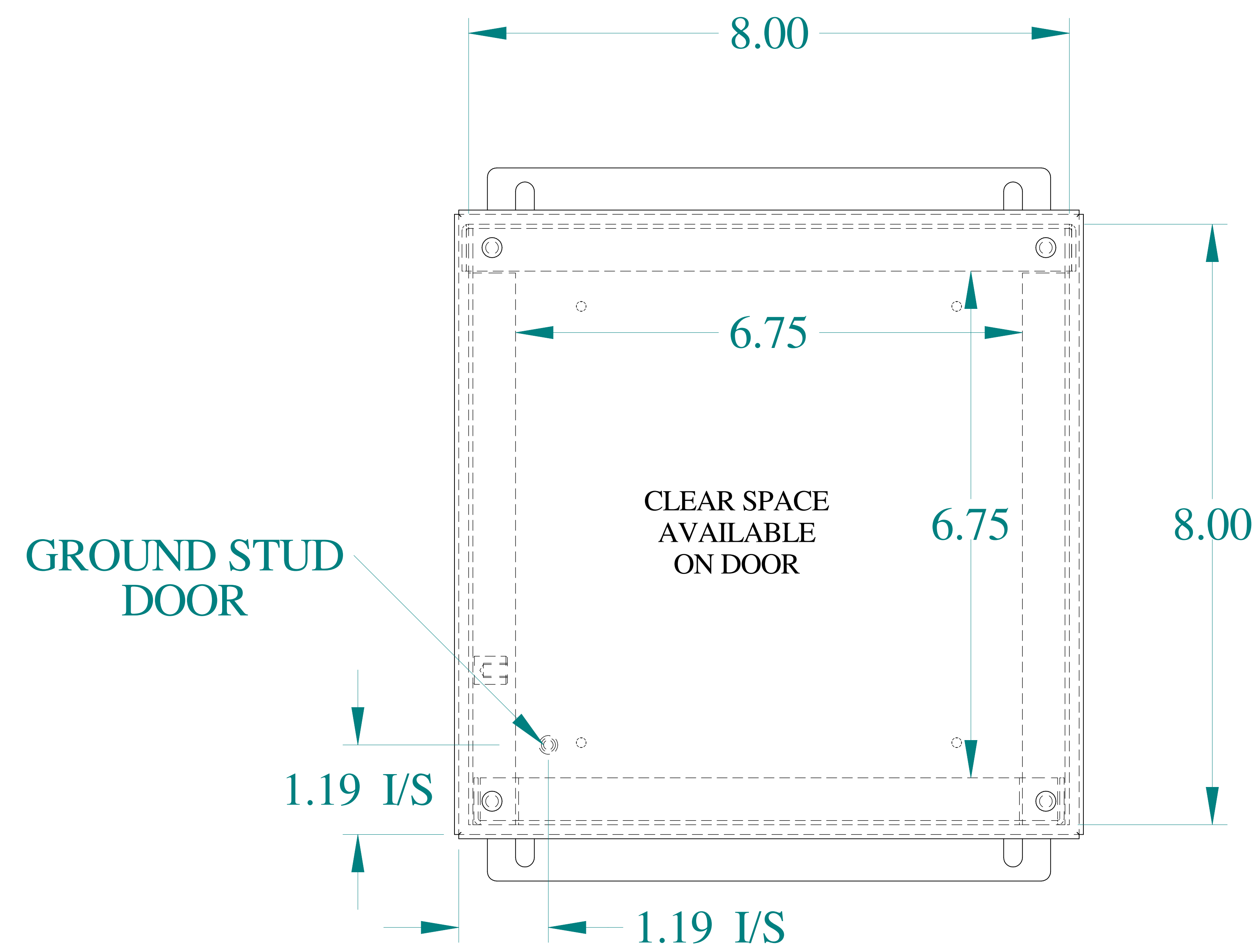
FRONT VIEW
