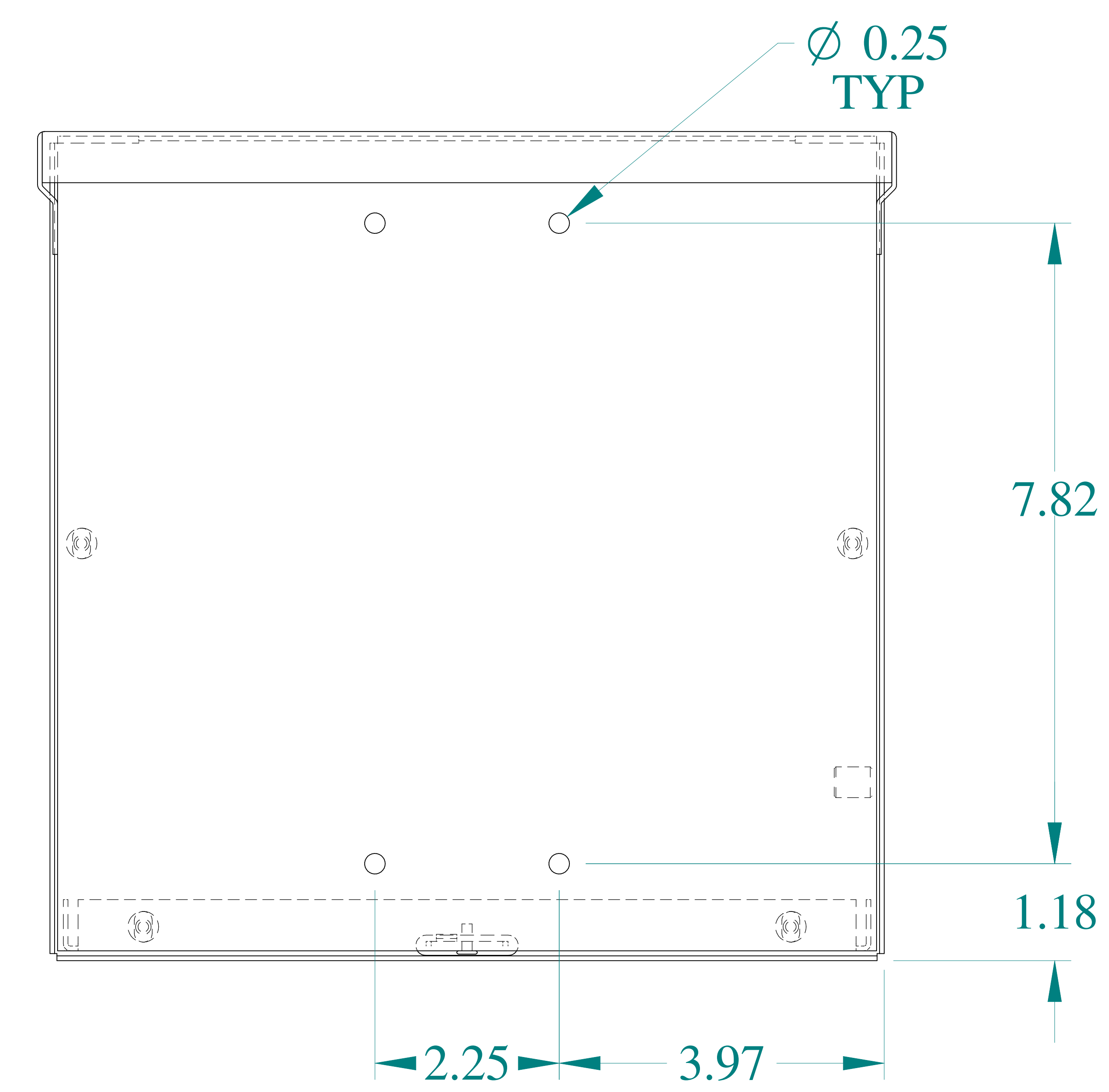
BACK VIEW
