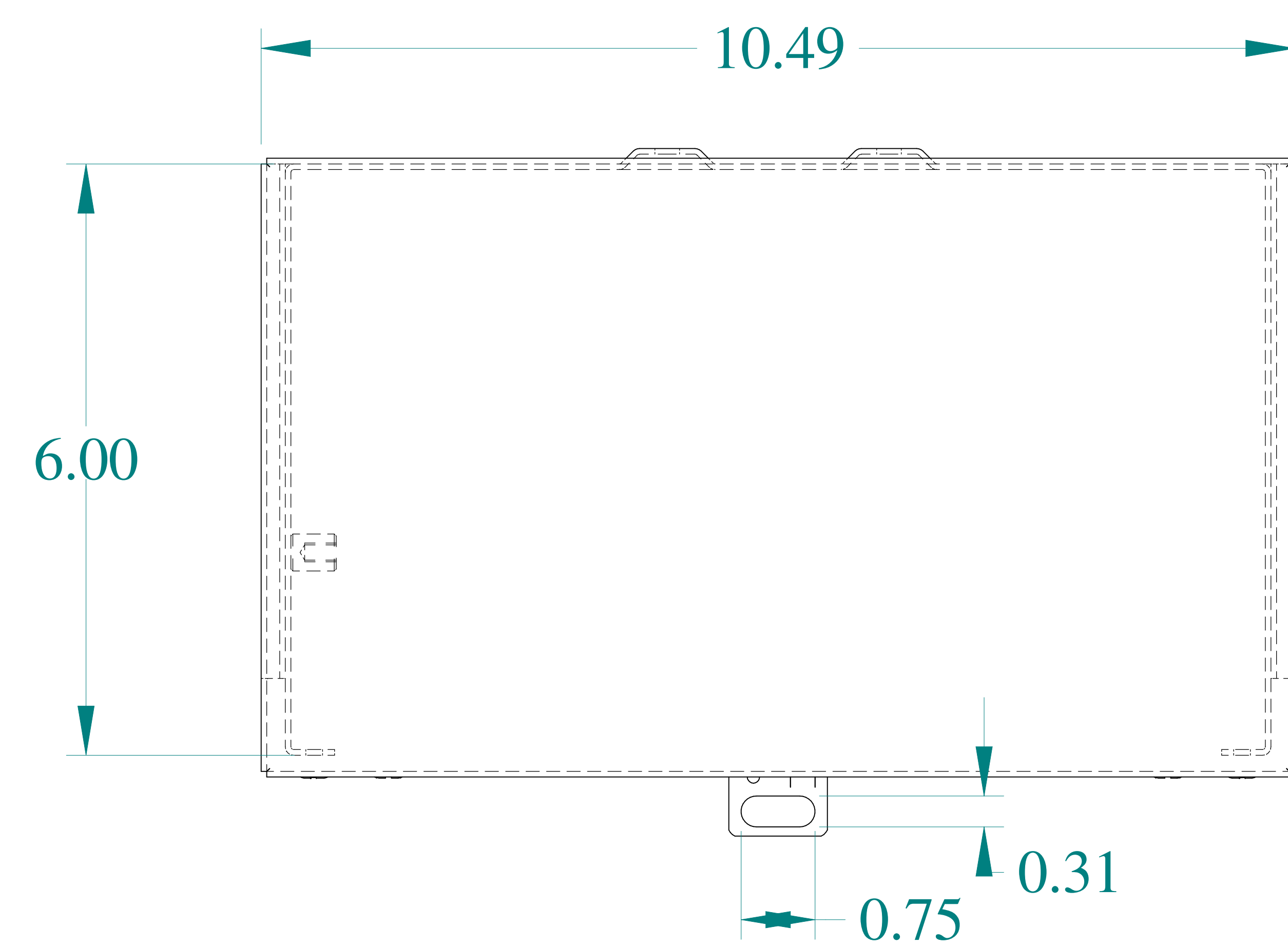
TOP VIEW
