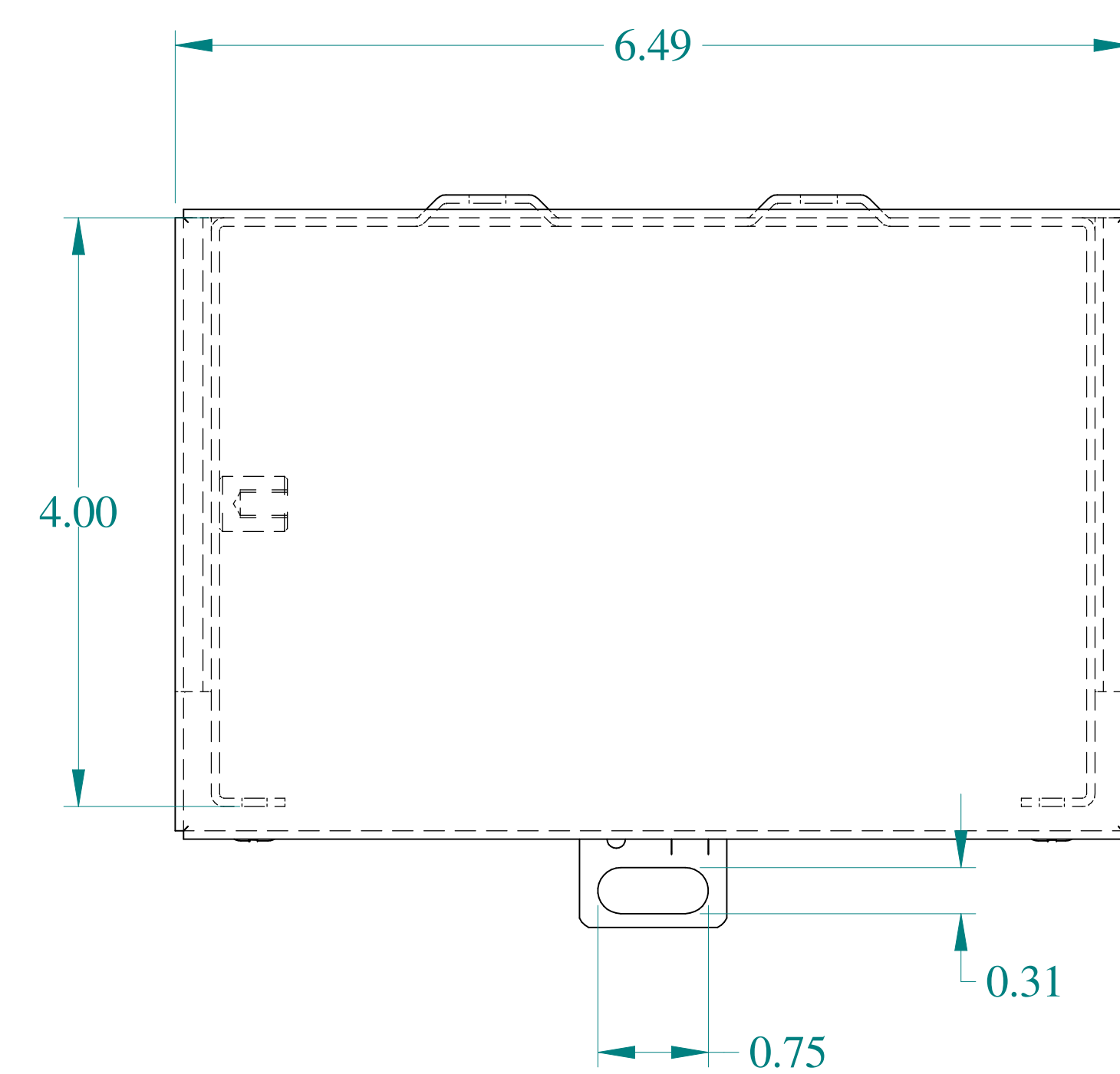
TOP VIEW
