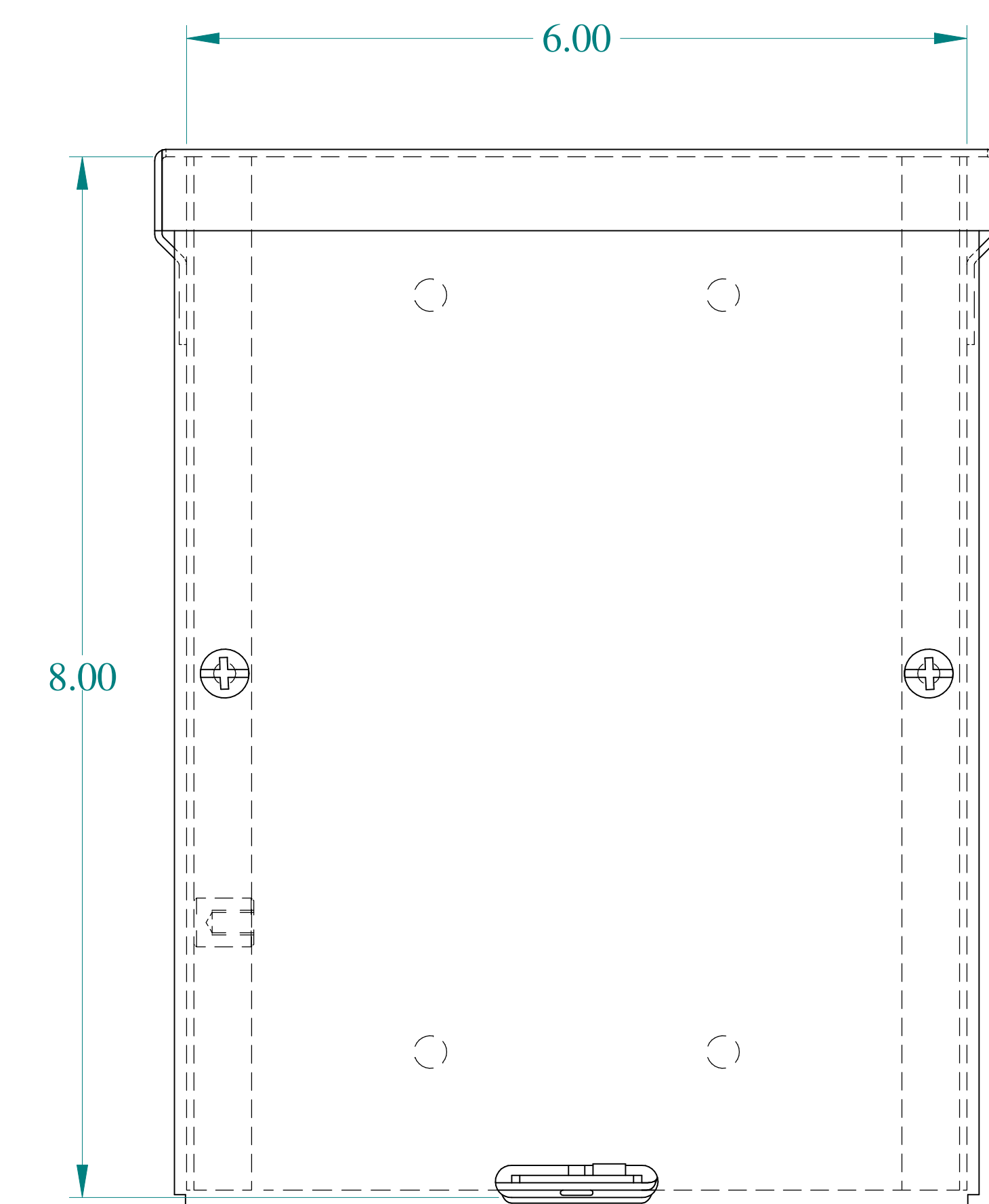
FRONT VIEW
