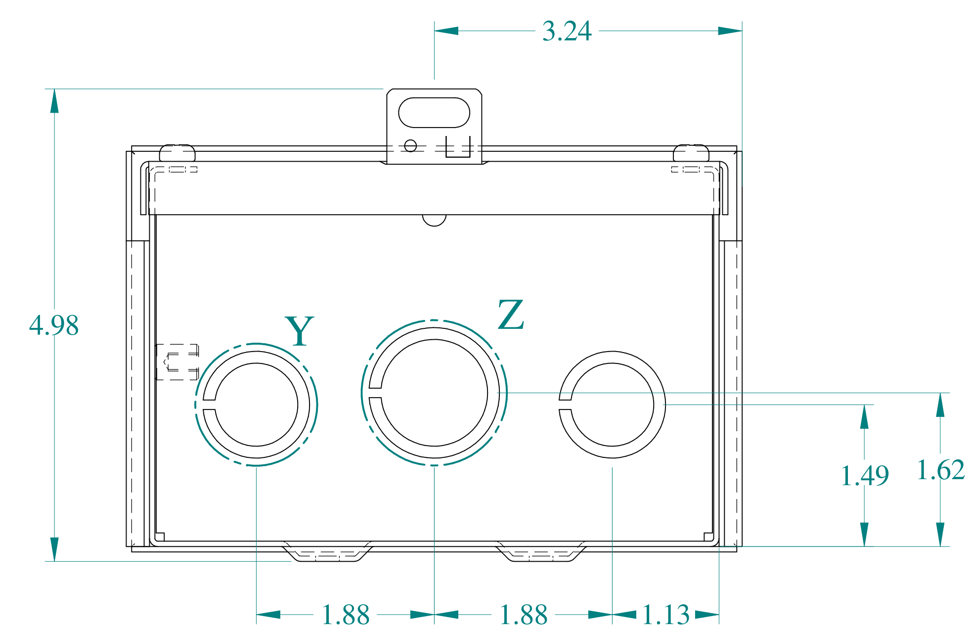
BOTTOM VIEW
