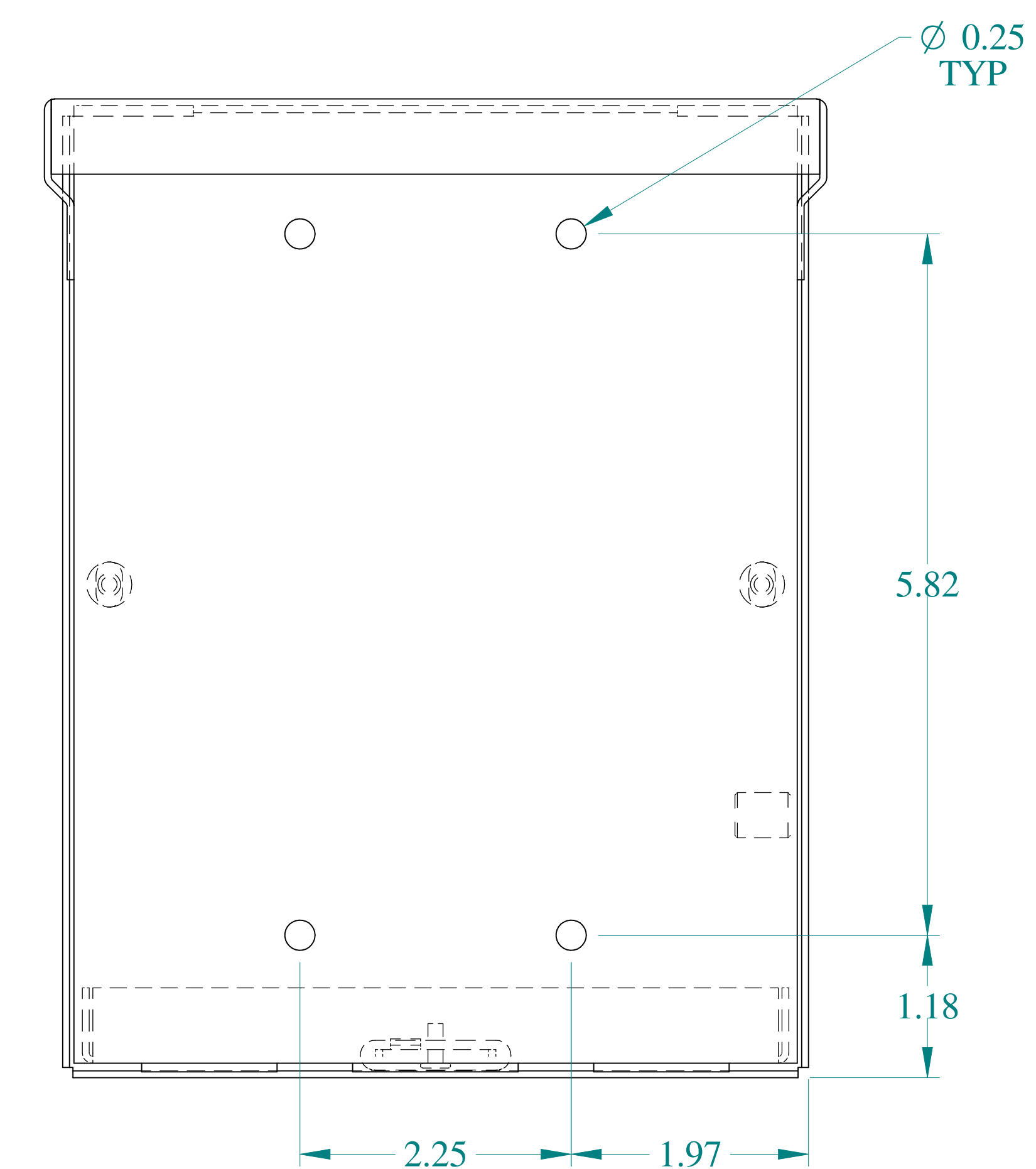
BACK VIEW
