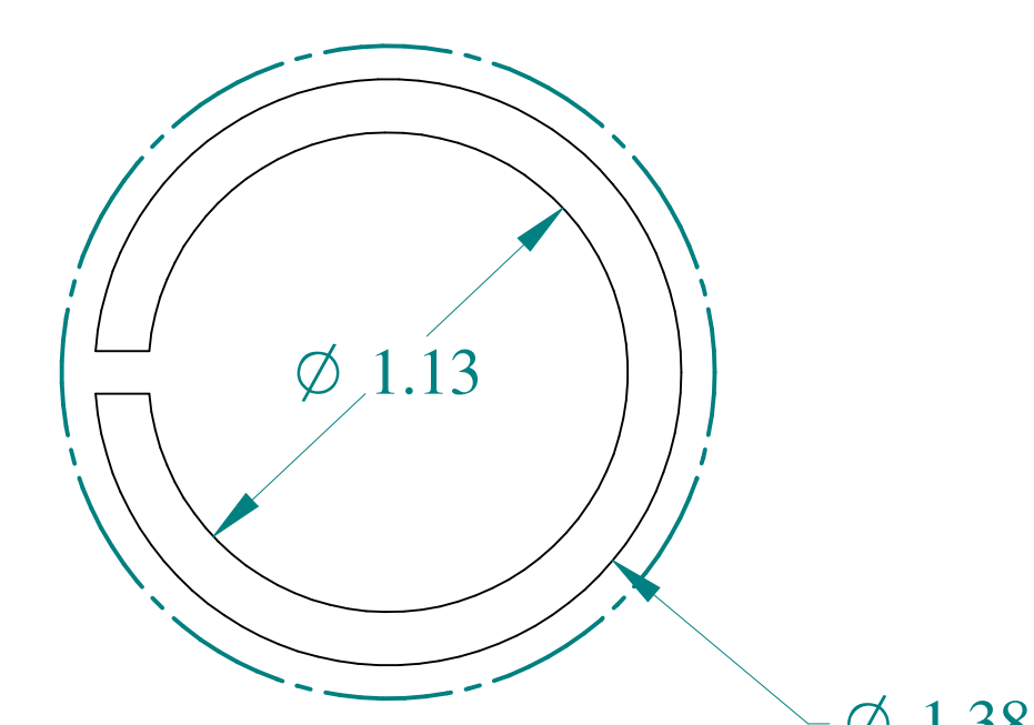
DETAIL Z
