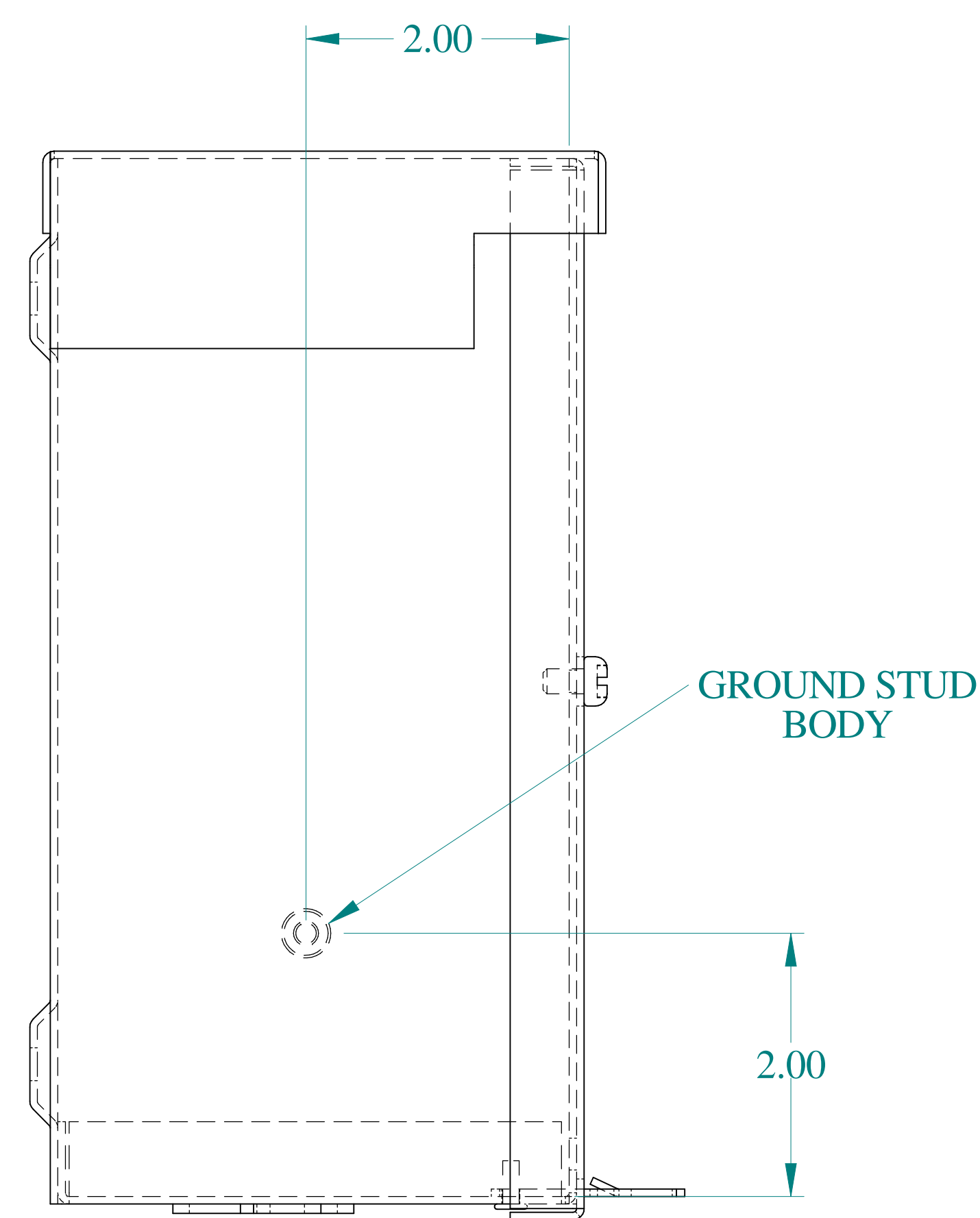
SIDE VIEW
