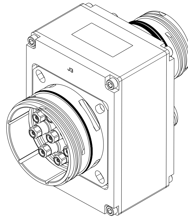
REAR ISOMETRIC VIEW SCALE 1.000
