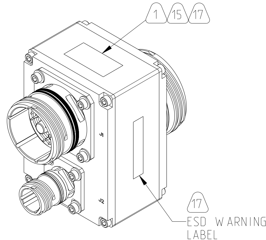
FRONT ISOMETRIC VIEW SCALE 1.000
