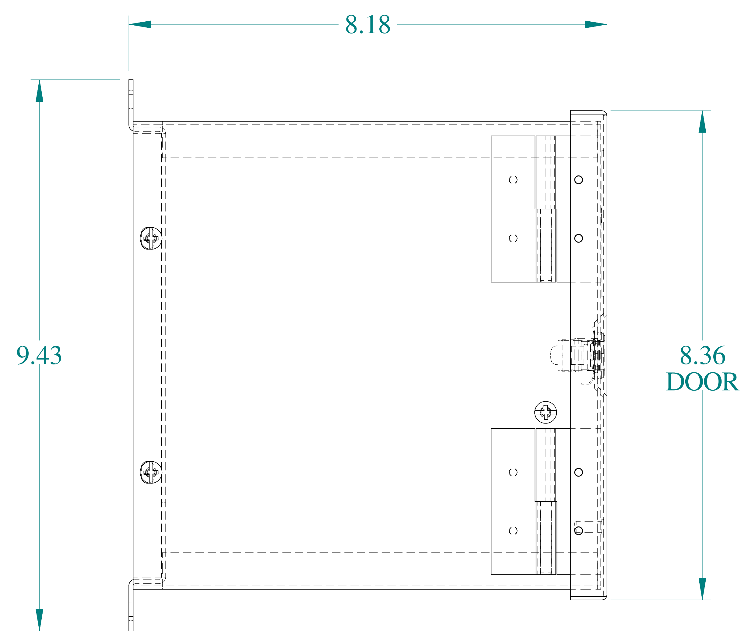
SIDE VIEW
