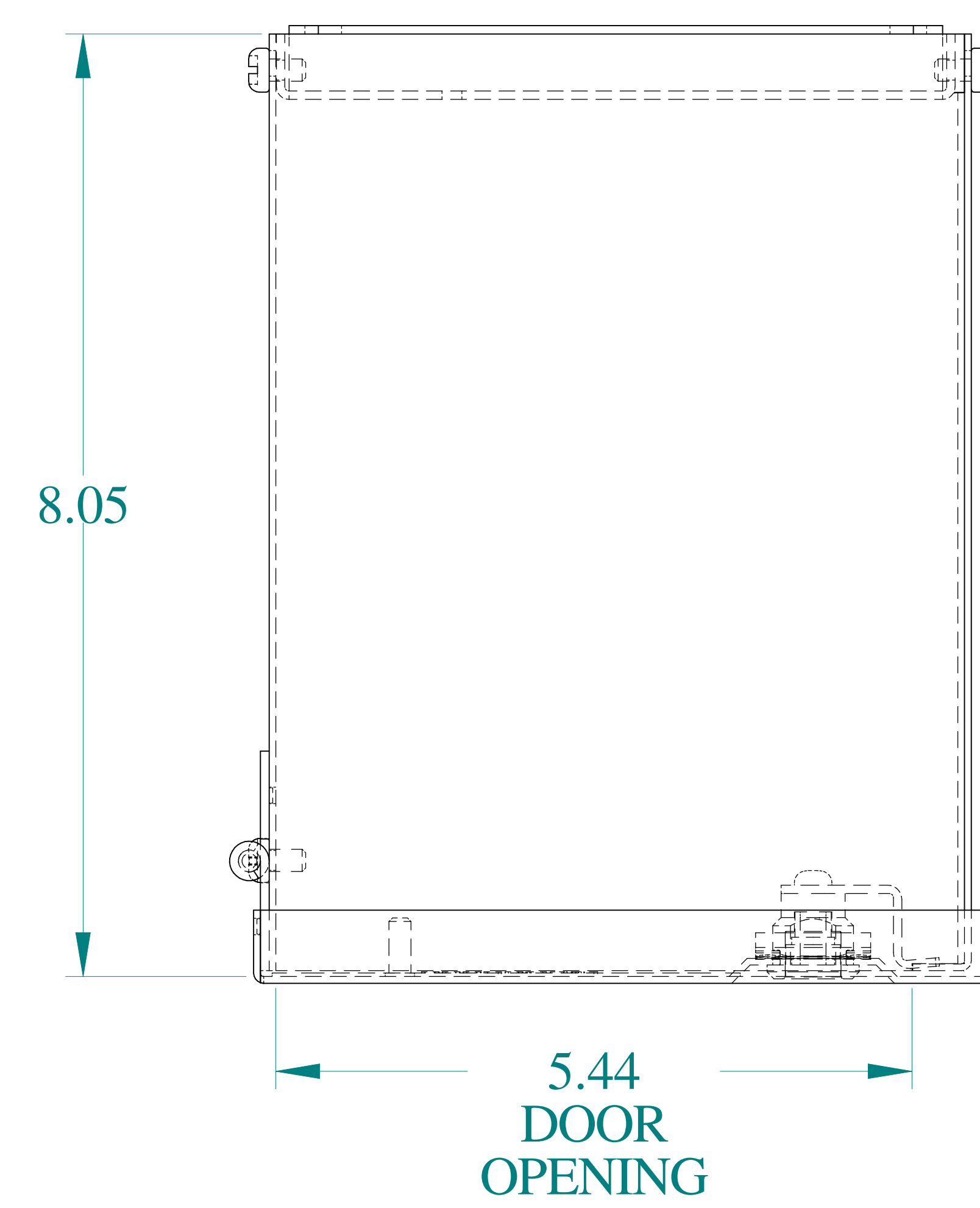
TOP VIEW
