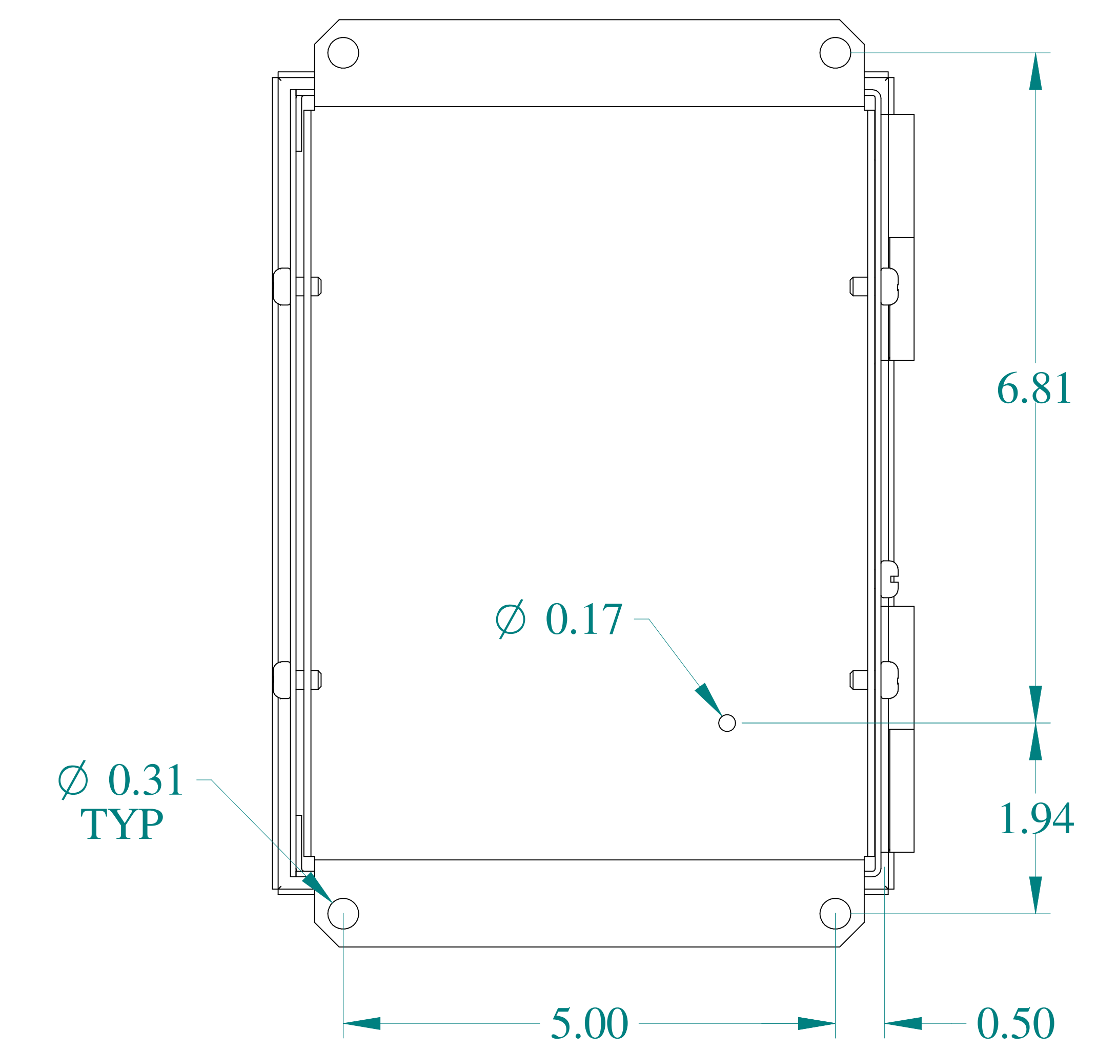
BACK VIEW
