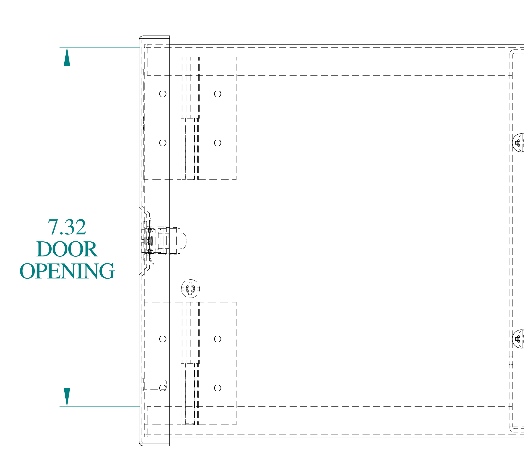
SIDE VIEW
