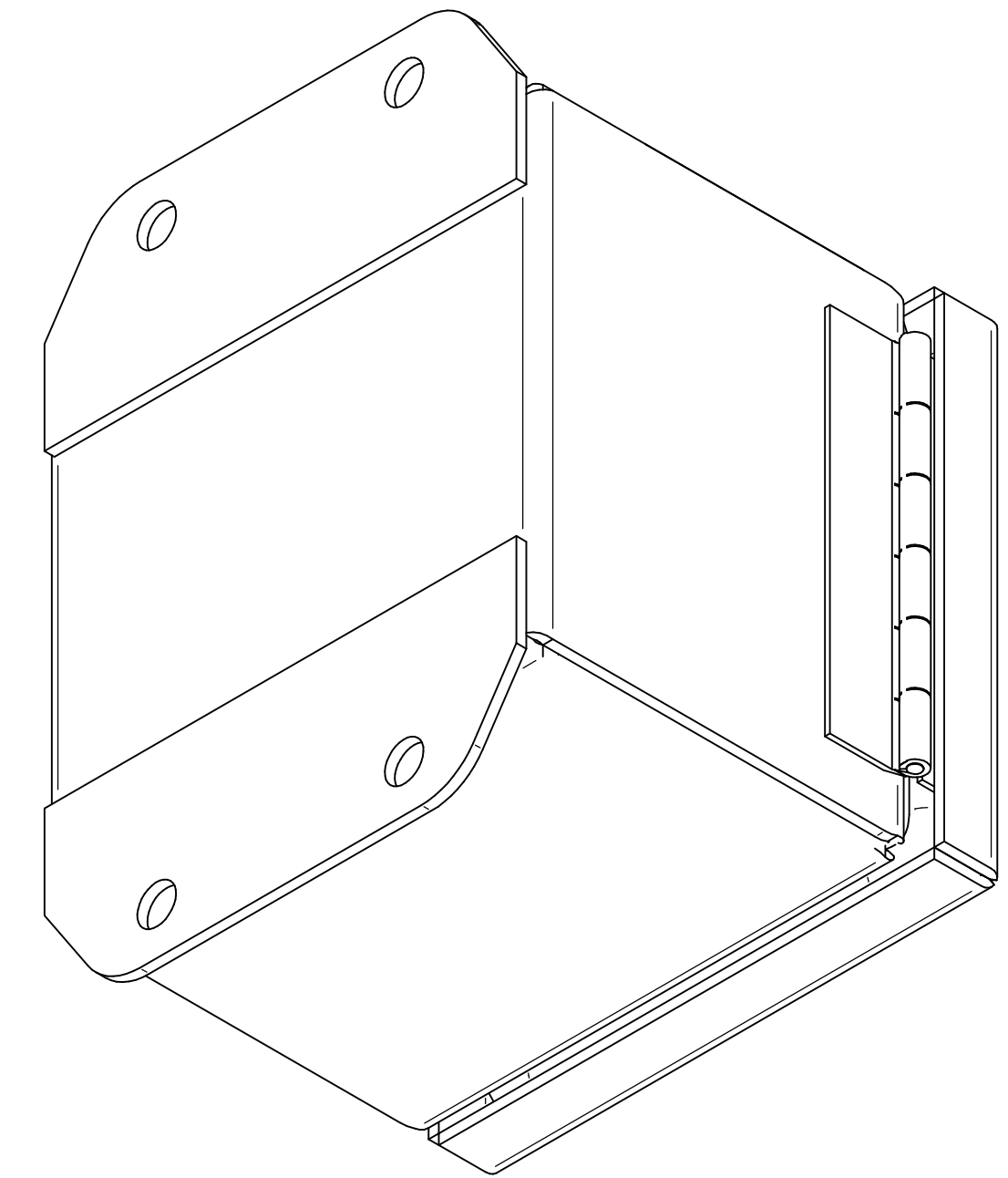
ISOMETRIC VIEWS
