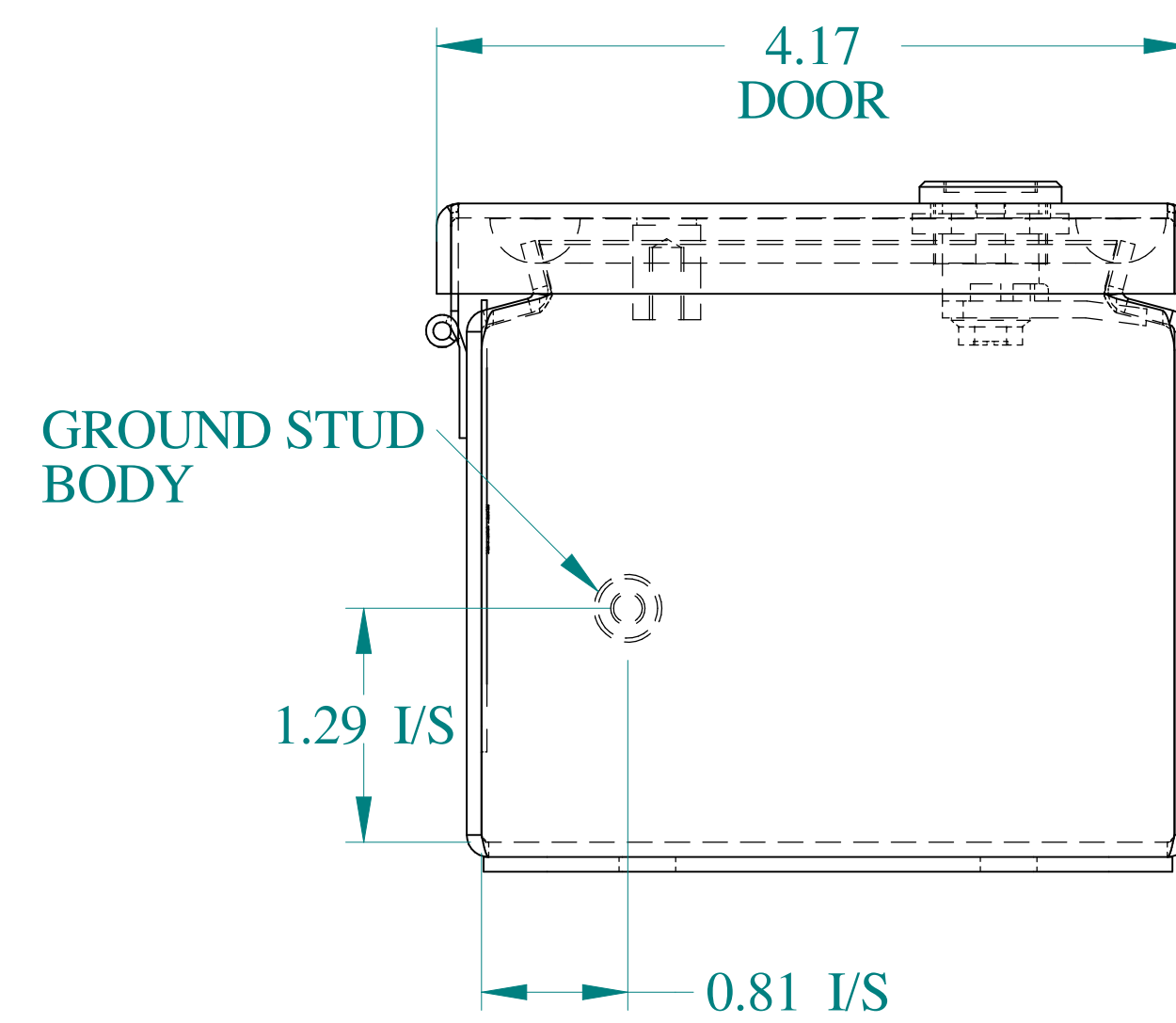
BOTTOM VIEW
