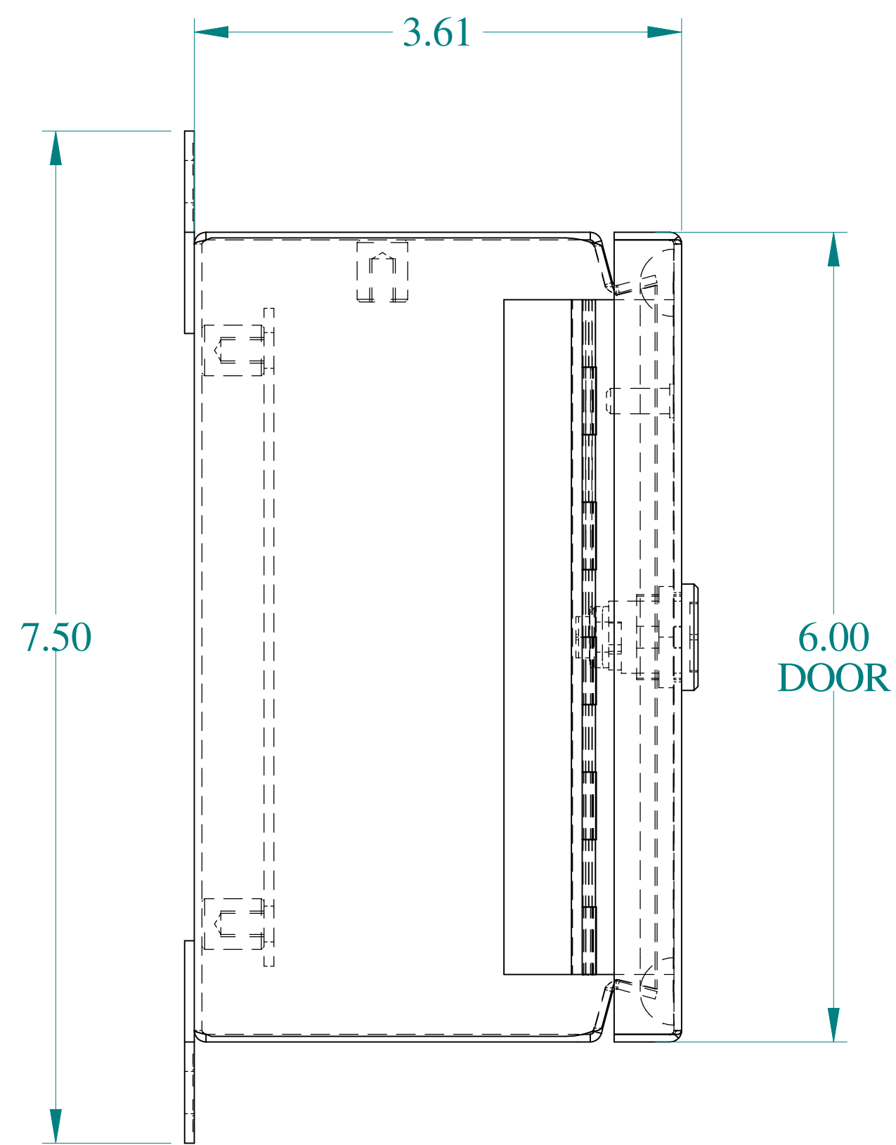
SIDE VIEW
