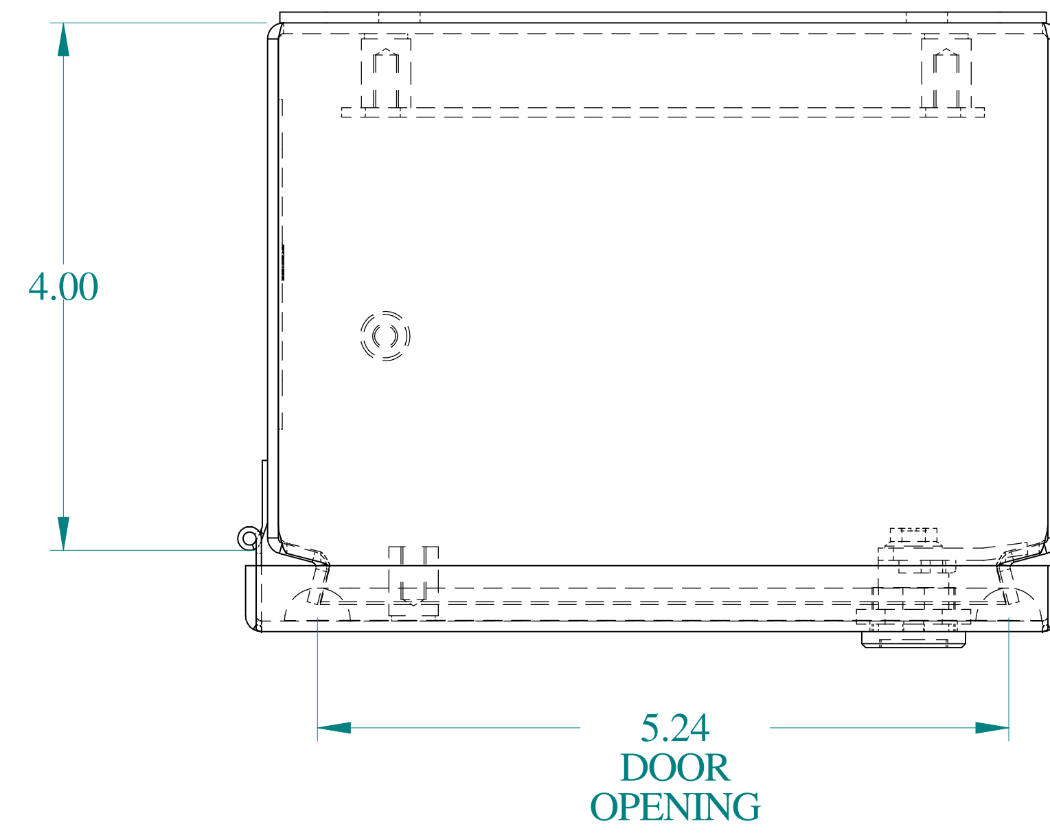
TOP VIEW
