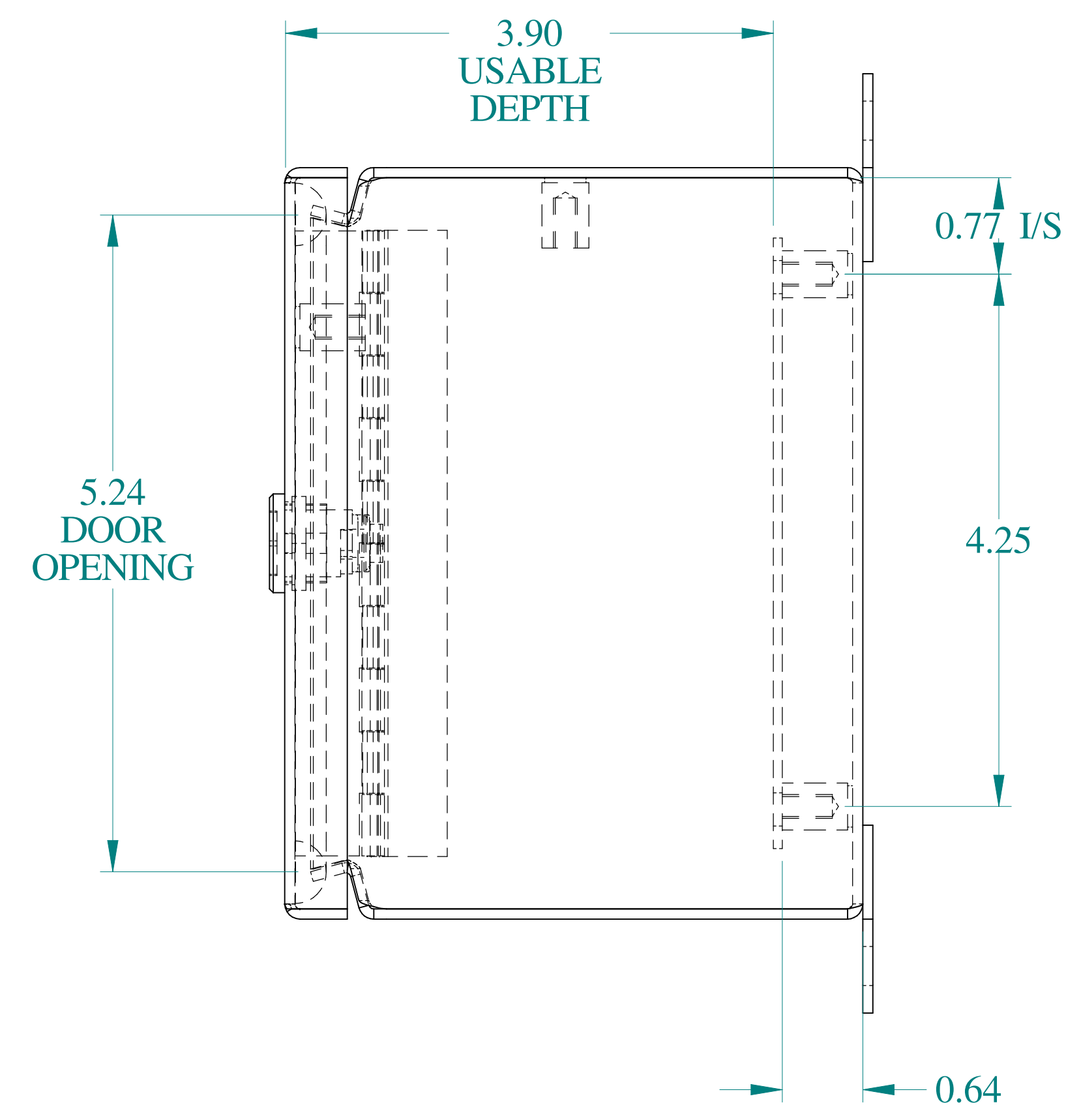
SIDE VIEW
