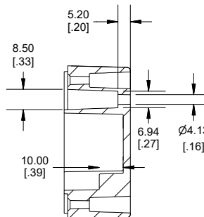
SECTION C-C MOUNTING HOLE
