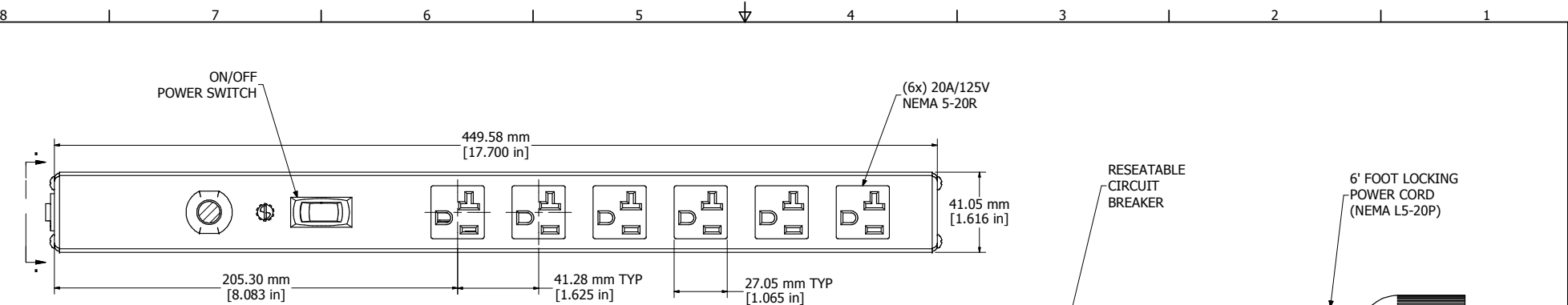
SECTION A-A (VIEW FROM FRONT)
