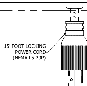
ASSEMBLY - VIEW FROM BOTTOM
