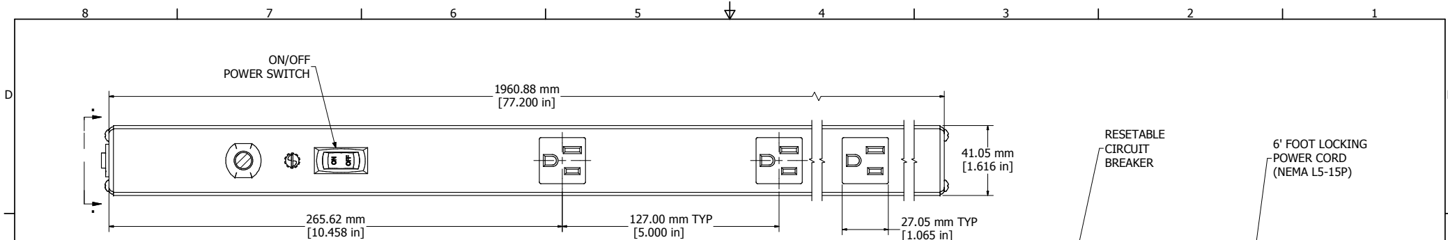
SECTION A-A (VIEW FROM FRONT)
