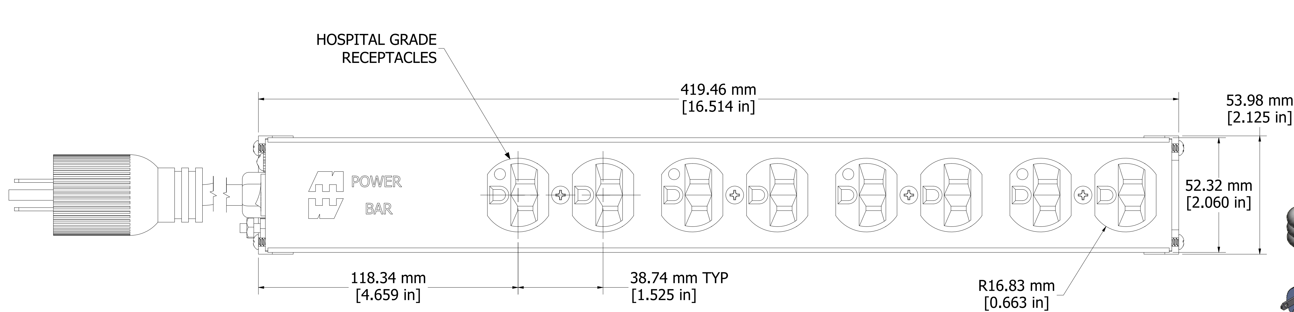
ASSEMBLY - VIEW FROM TOP
