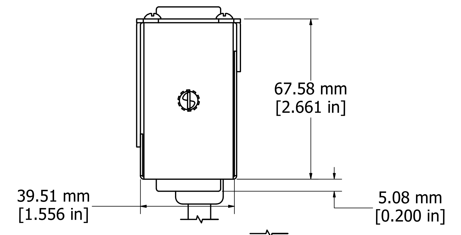
ASSEMBLY - VIEW FROM SIDE
