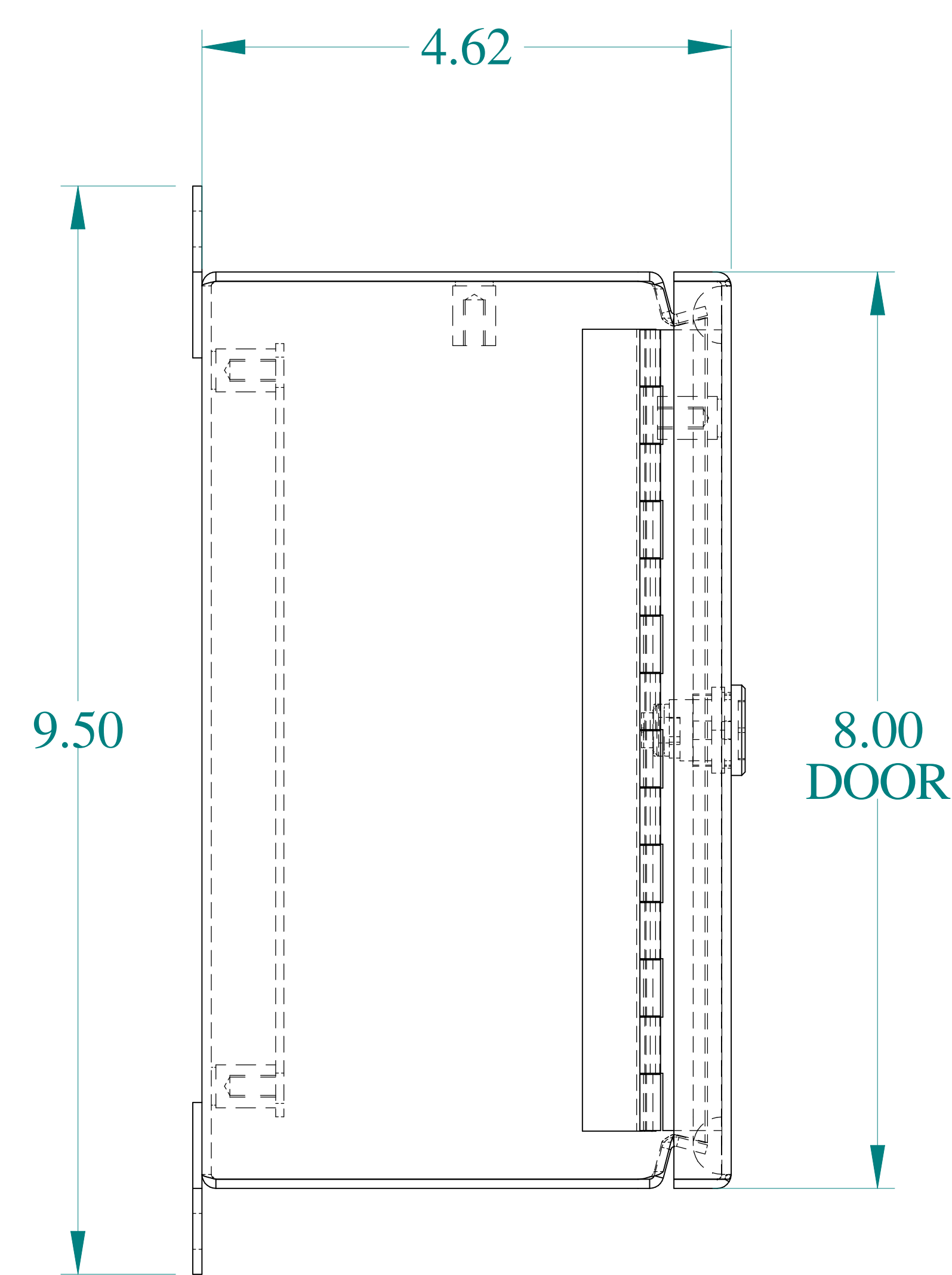
SIDE VIEW
