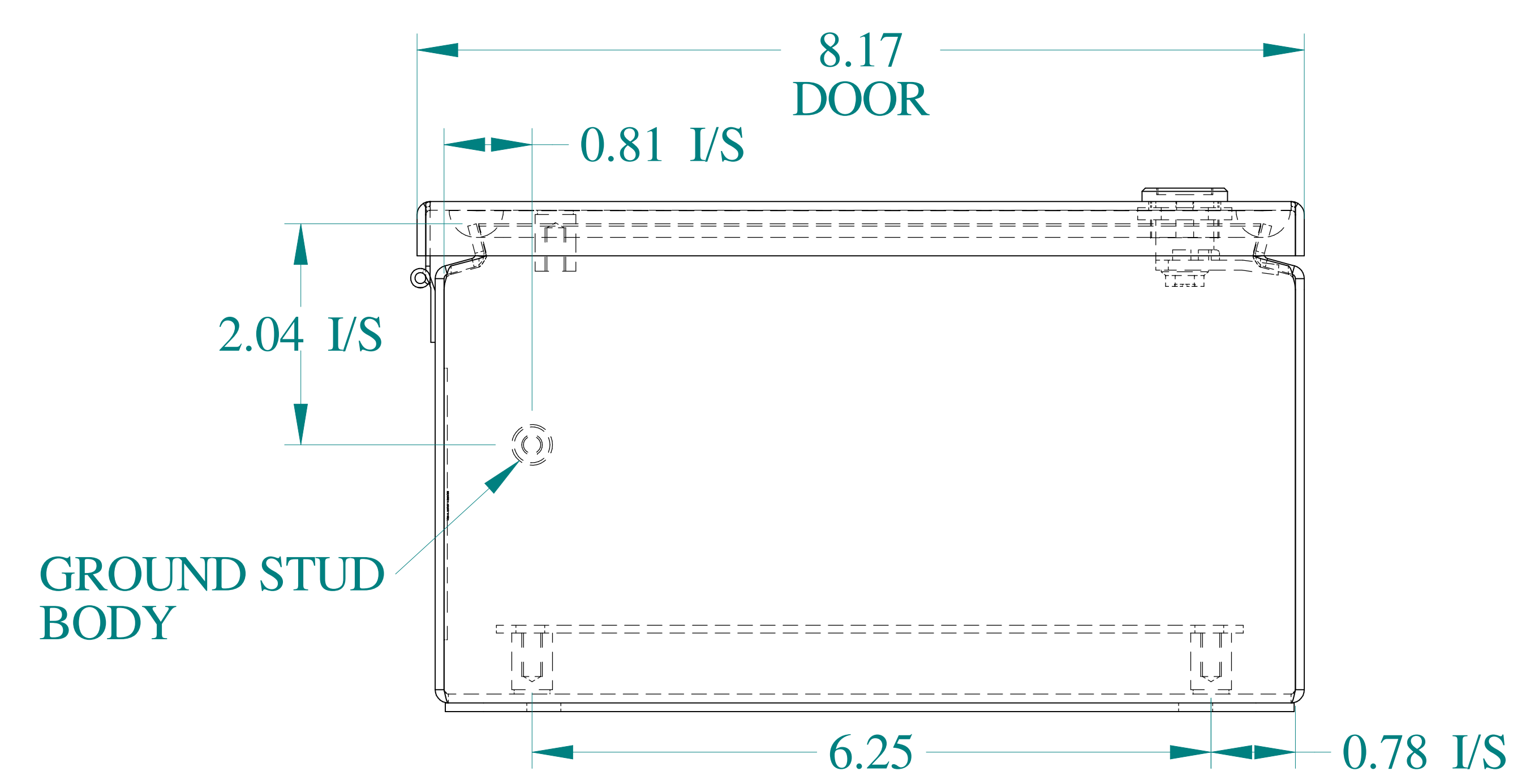
BOTTOM VIEW
