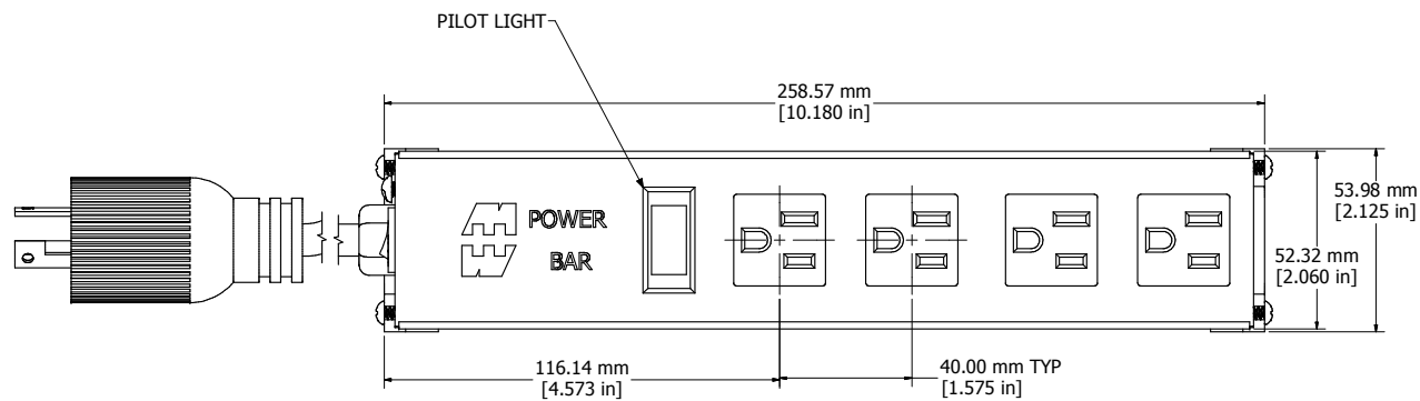
ASSEMBLY - VIEW FROM TOP
