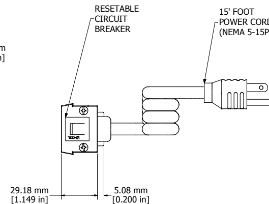
ASSEMBLY - VIEW FROM END
