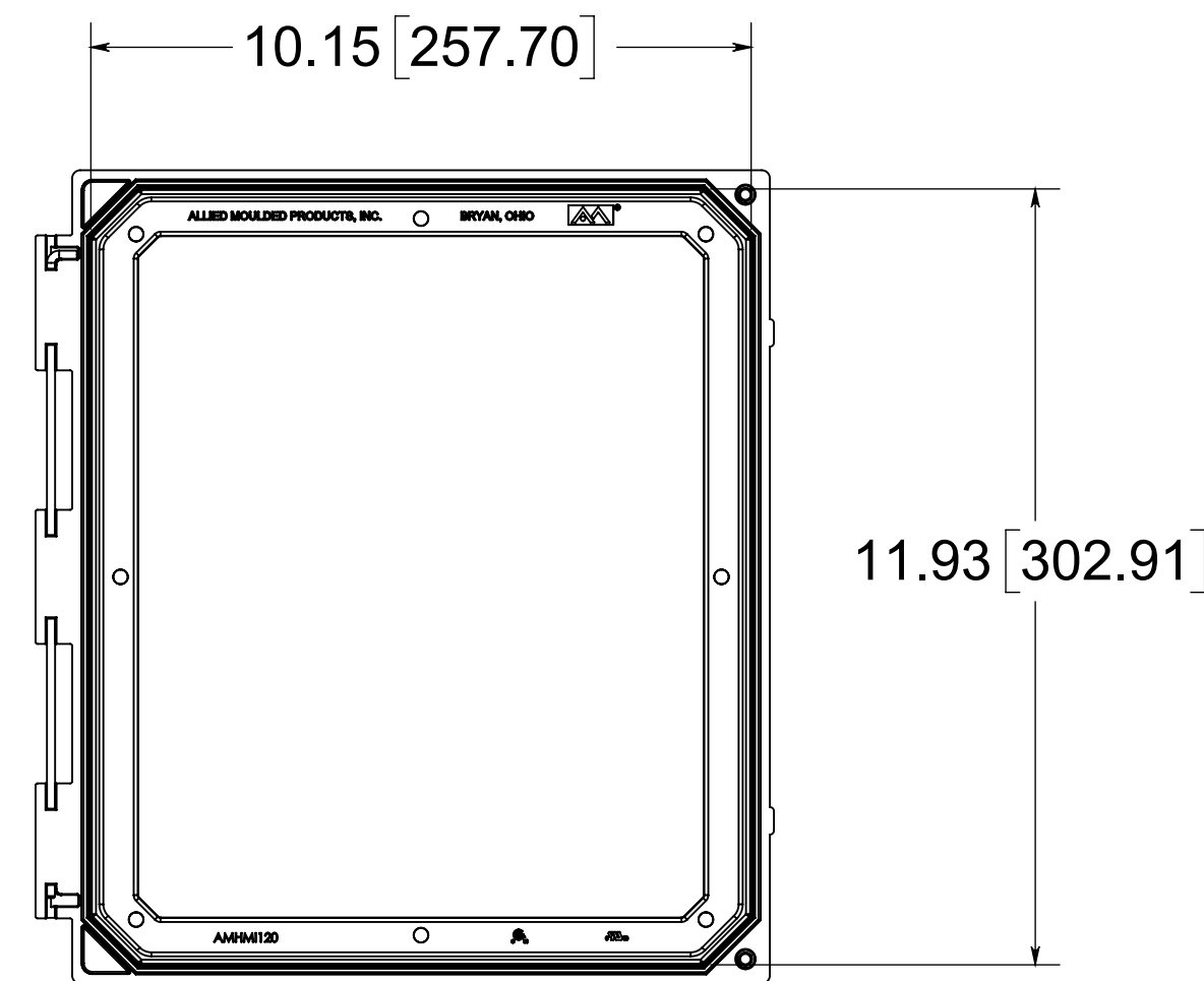
FRONT VIEW WITH COVER REMOVED
