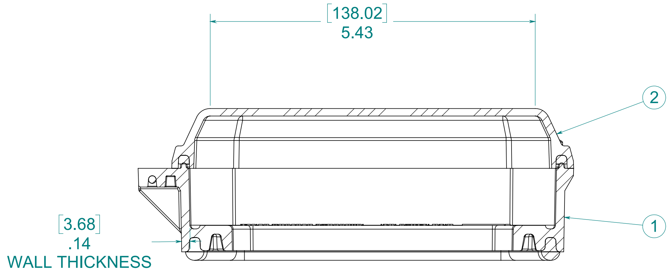
SECTION B-B
